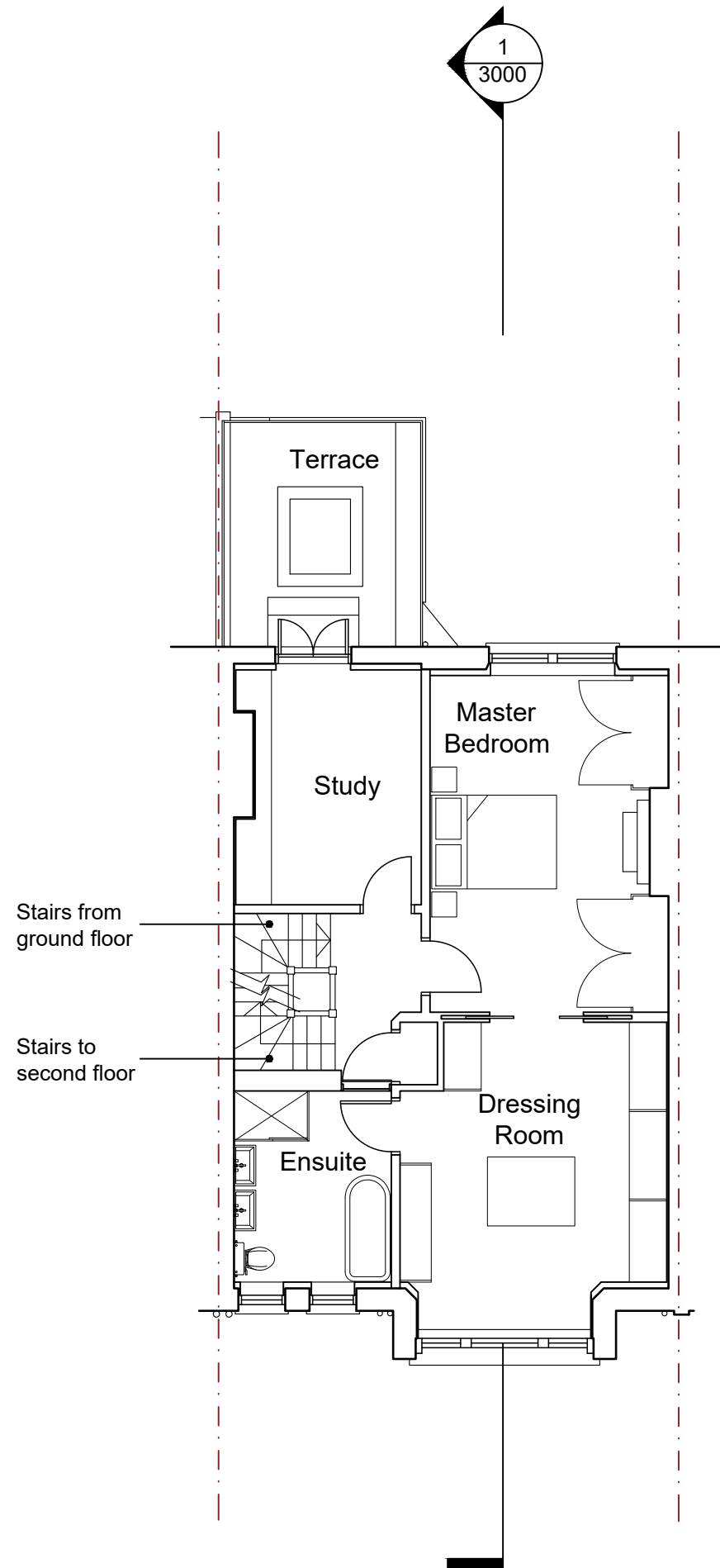
1 Proposed First Floor Plan - NO CHANGES TO LAYOUT 1:100
