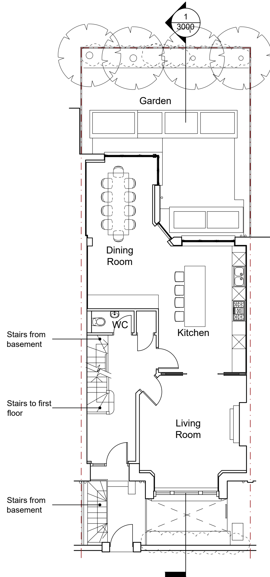
1 Proposed Ground Plan - NO CHANGES TO LAYOUT 1:100
