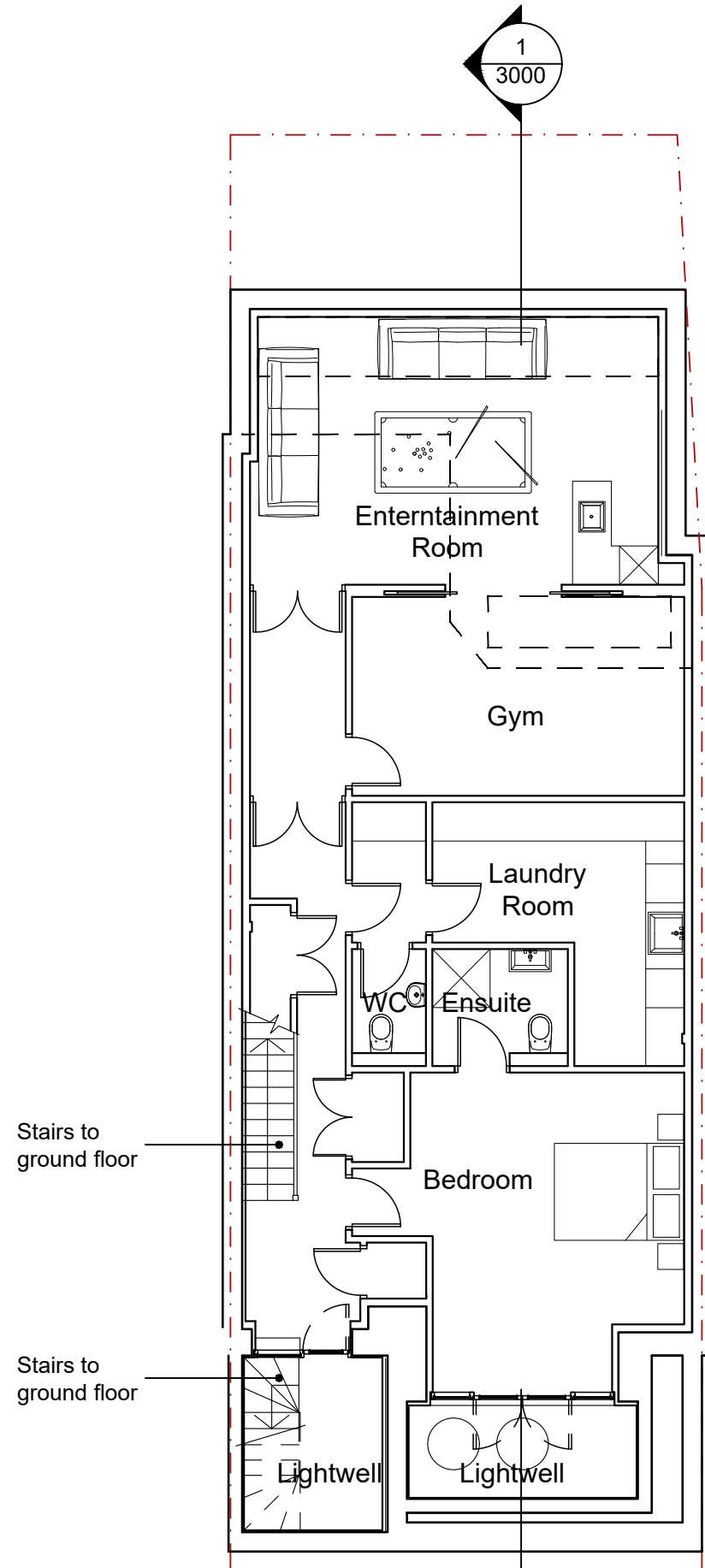
1 Proposed Basement Plan - NO CHANGES TO LAYOUT 1:100
