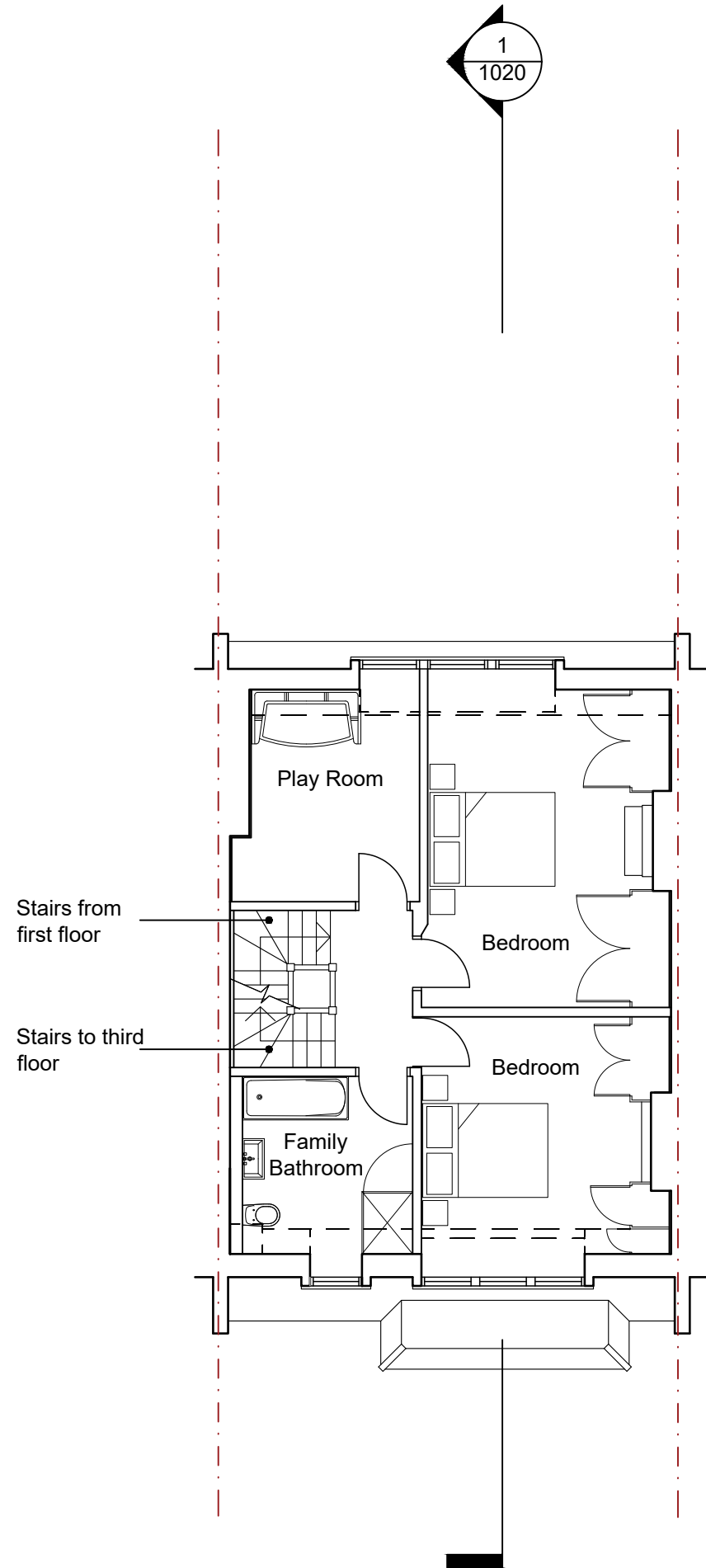
1 Existing Second Floor Plan 1:100
