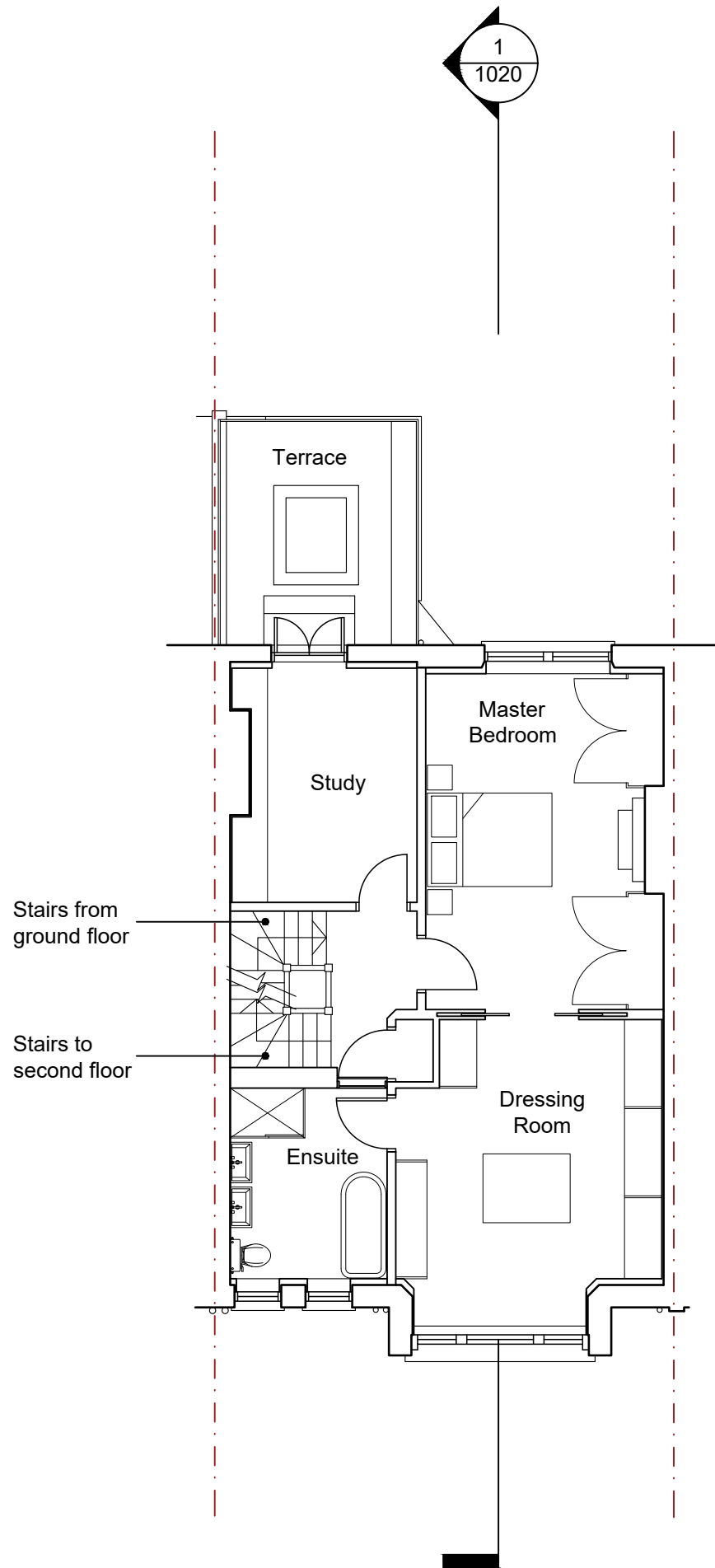
1 Existing First Floor Plan 1:100
