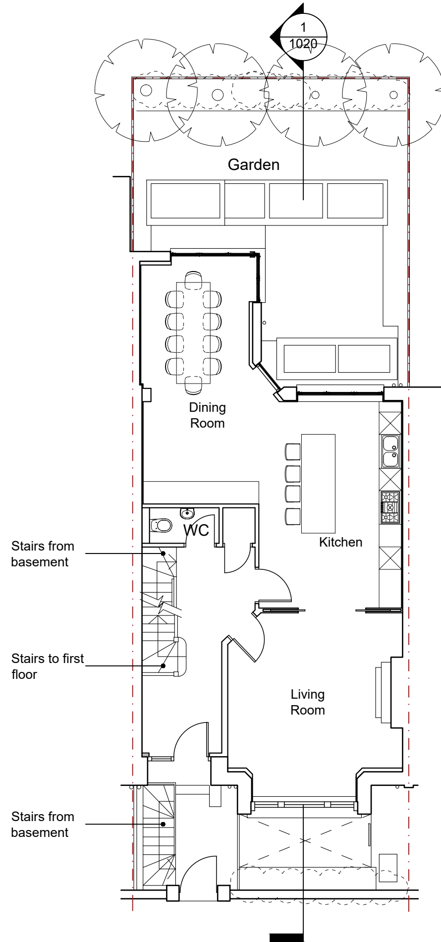
1 Existing Ground Plan 1:100
