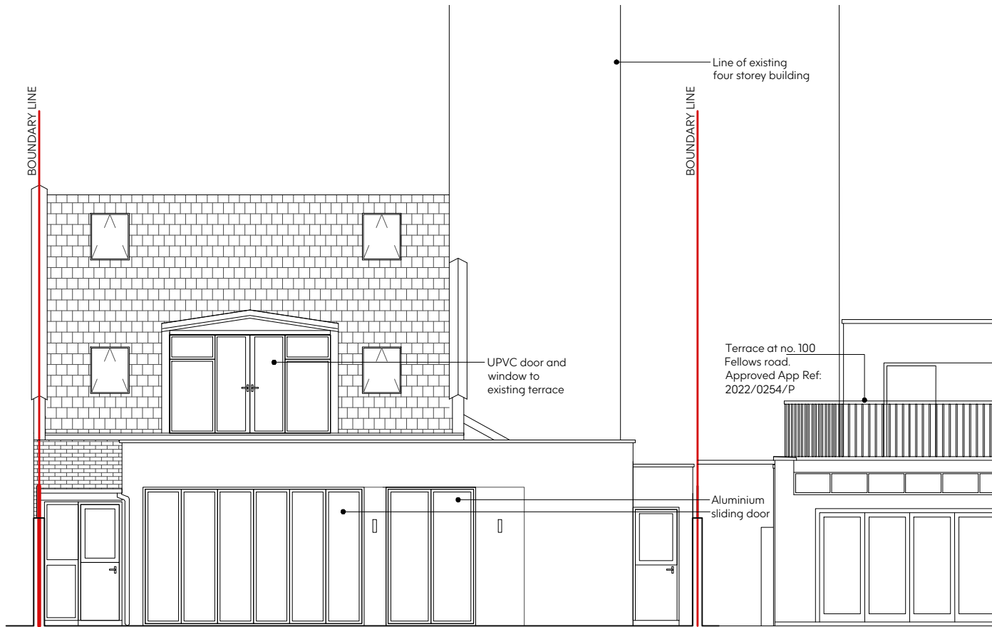
① Existing Rear Elevation Scale 1:100
