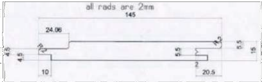
LT AC 02 - designed for vertical installation
