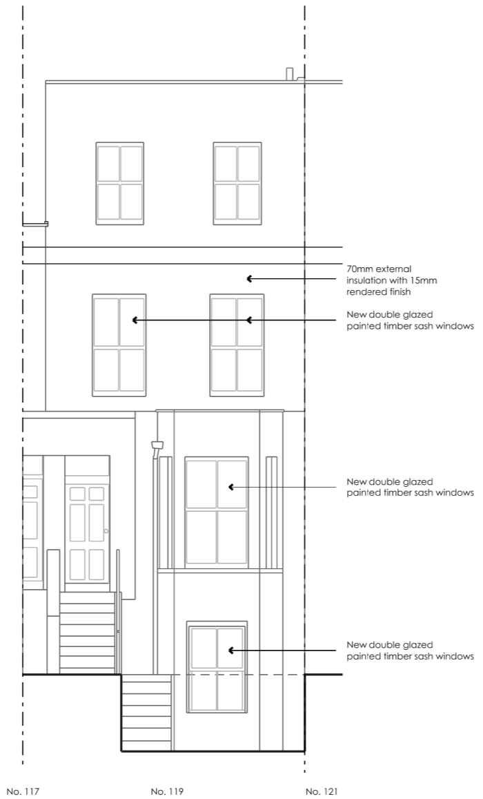
Proposed Front Elevation (No works)
