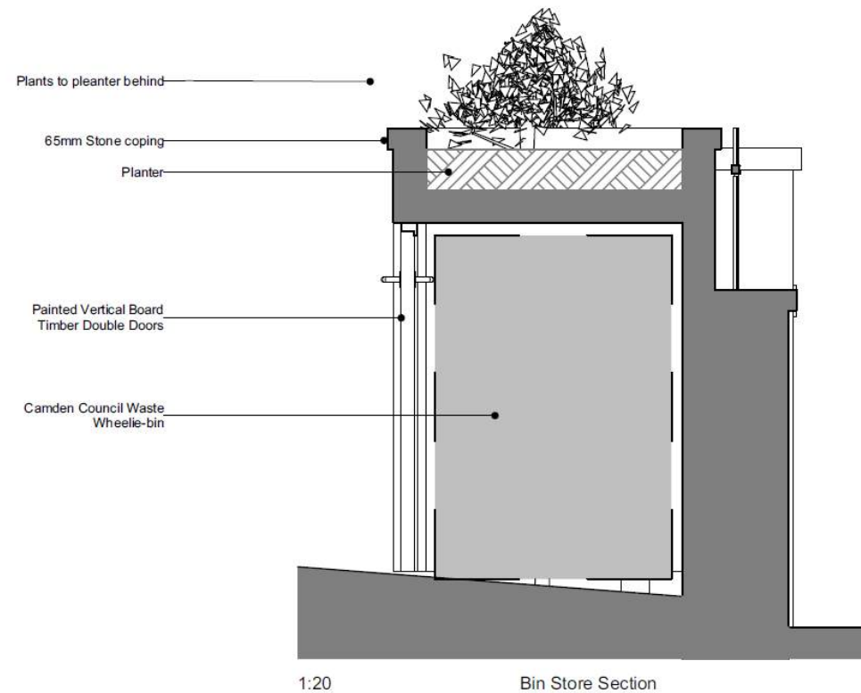
Architect typical elevation & section details
