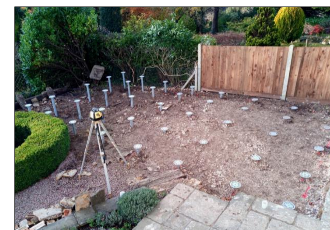
Typical Ground Screw Finished Installation
