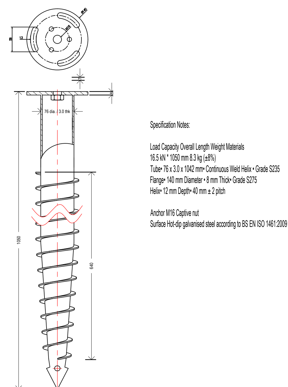
RDX PRO RF140 M16 76x1050-T3.0 Ground Screw @ 1:5
