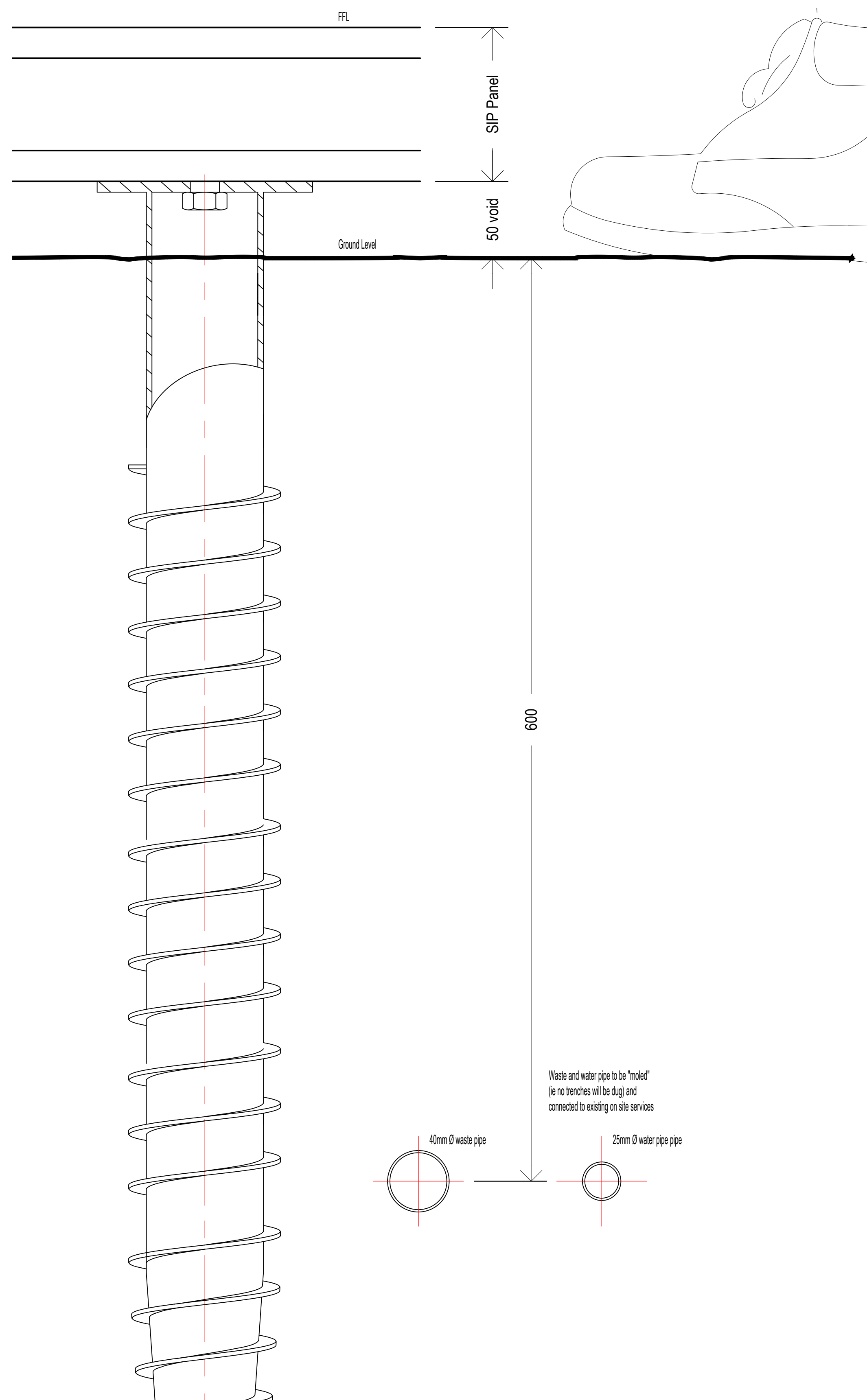
Ground Screw / Services Schematic Detail @ 1:2
