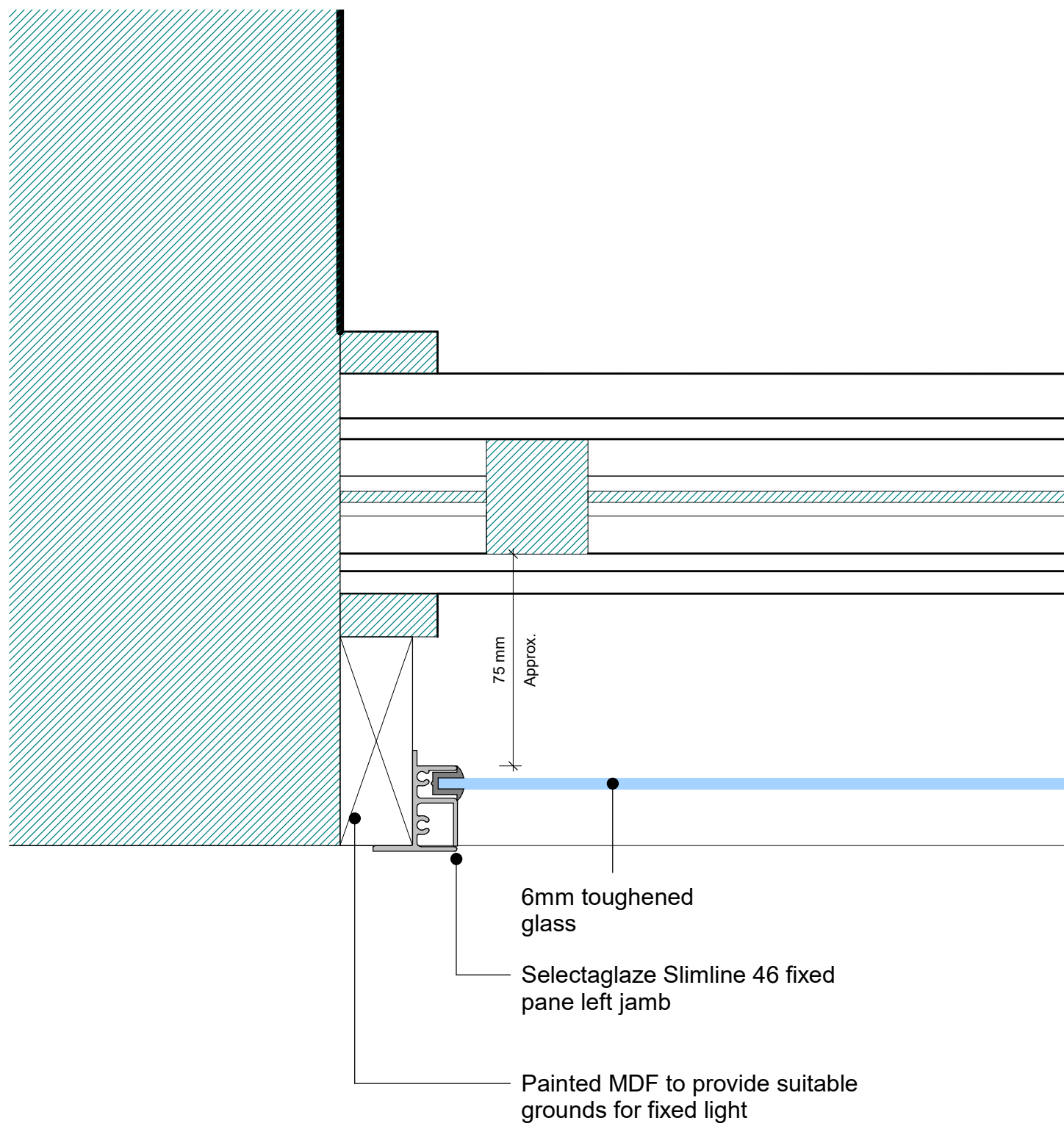
4503_First Floor_Plan_Detail_Secondary Glazing Fixed Panel Left Jamb
