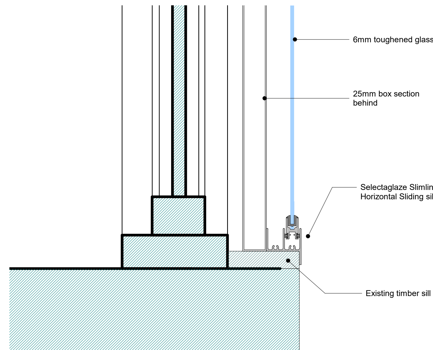
4503_First Floor_Section_Detail_Secondary Glazing Detail Sill
