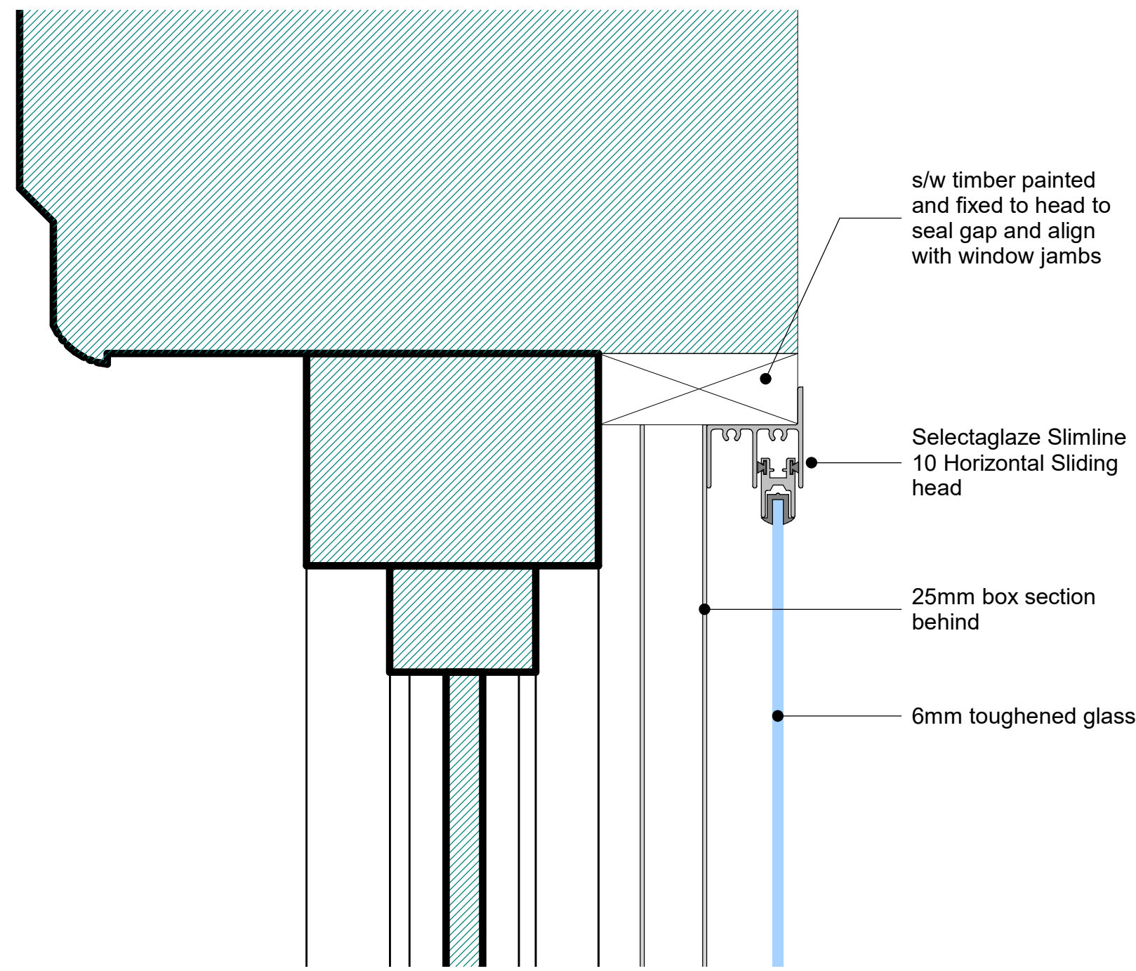
4503_First Floor_Section_Detail_Secondary Glazing Detail Head
