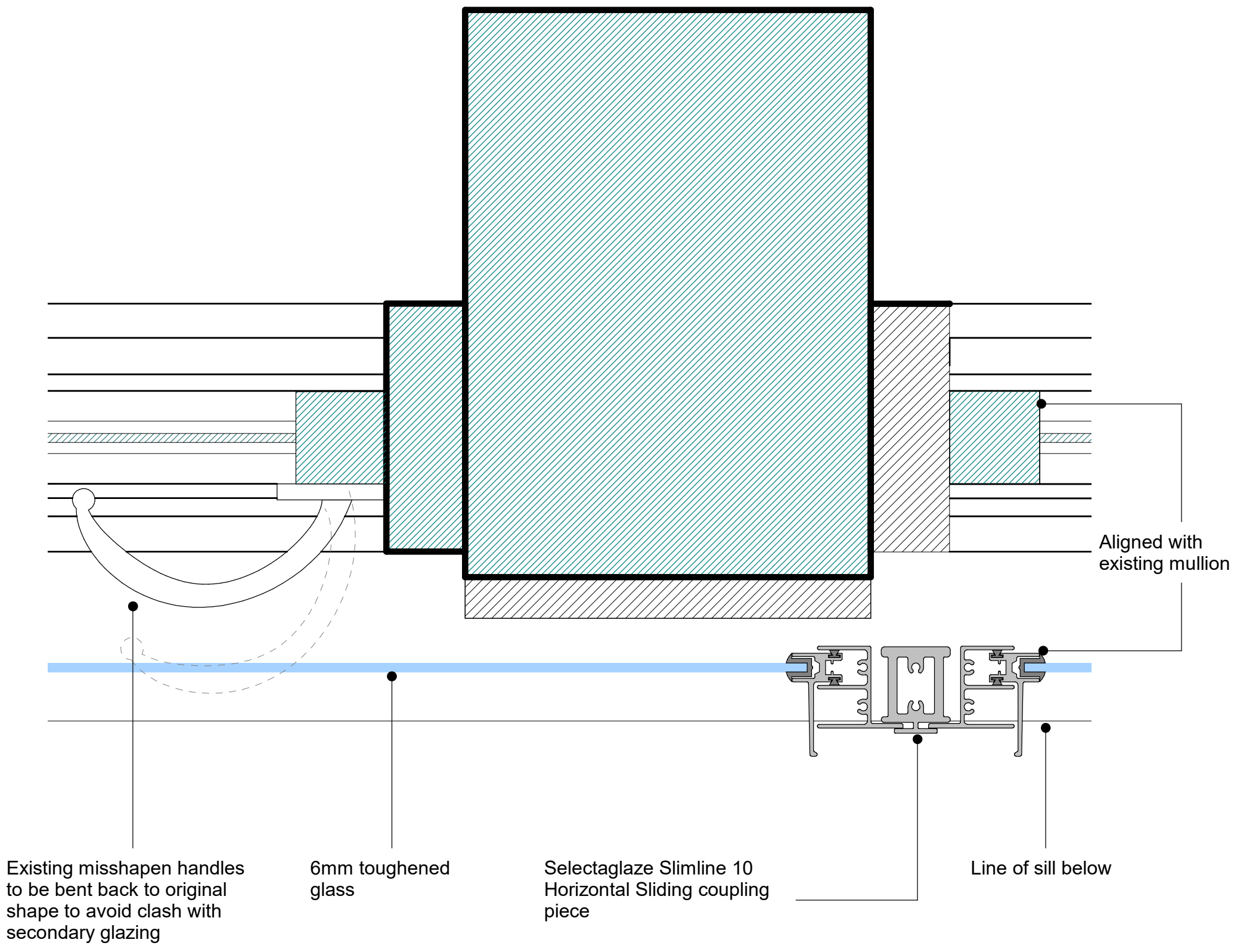
4503_First Floor_Plan_Detail_Secondary Glazing Coupling Piece
