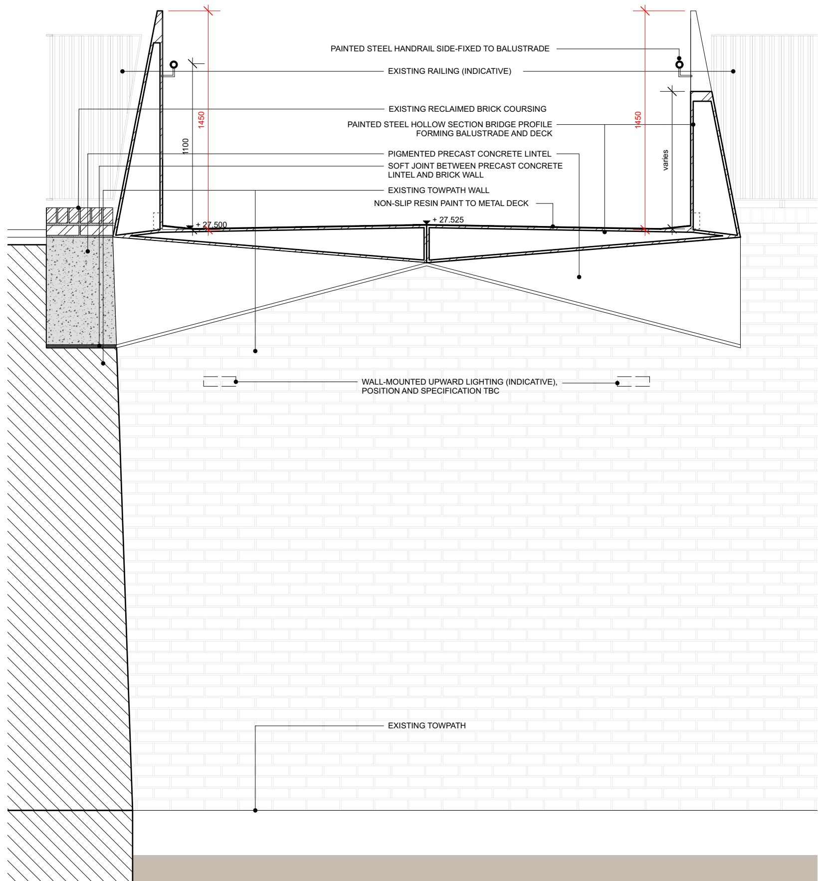
03 CROSS SECTION D-D' THROUGH TOWPATH WALL
