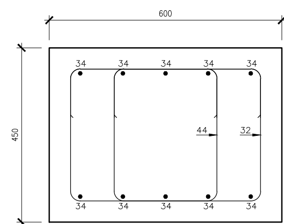
TYPICAL SECTION THROUGH STRIP FOUNDATION SCALE 1:10
