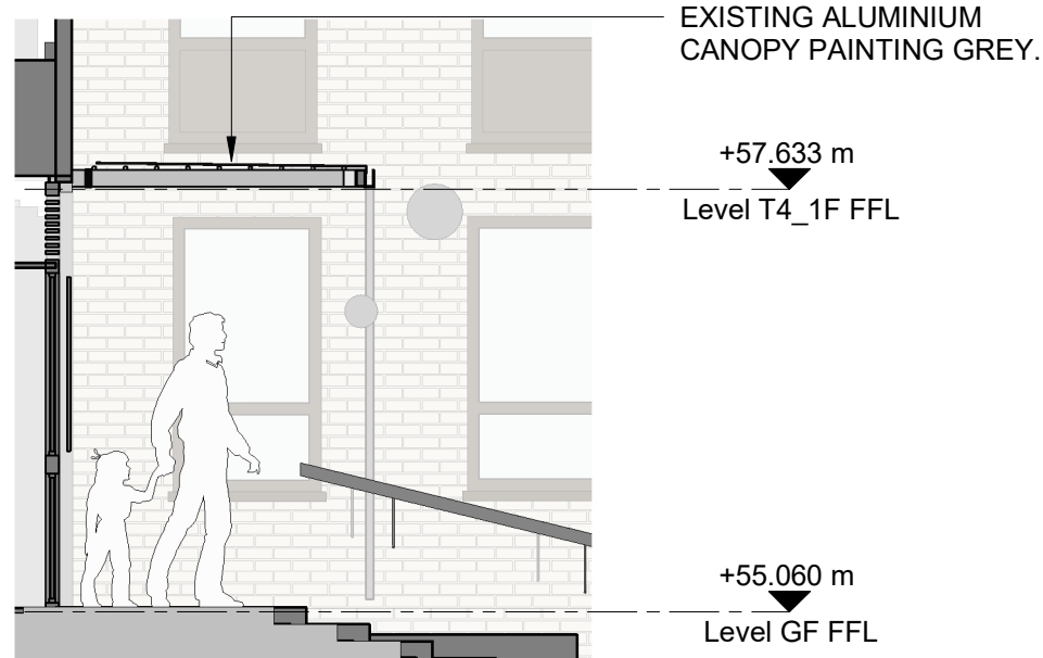
1 T4 - CANOPY 1 - EXISTING WEST ELEVATION 1 : 50
