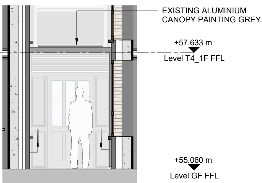
2 T4 - CANOPY 1 - EXISTING SOUTH ELEVATION 1 : 50
