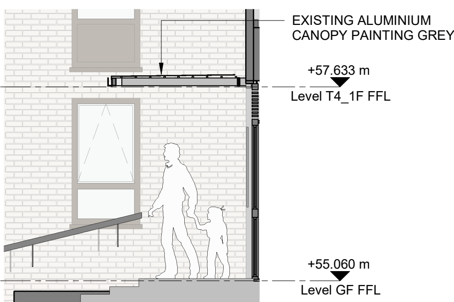
3 T4 - CANOPY 1 - EXISTING EAST ELEVATION 1 : 50
