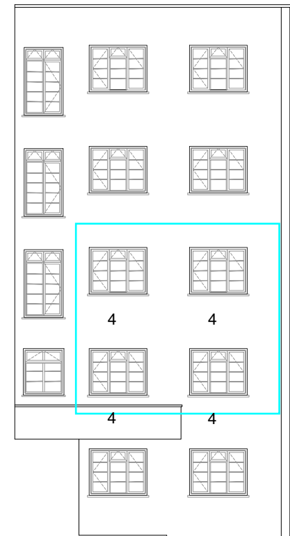
ELEVATION H
