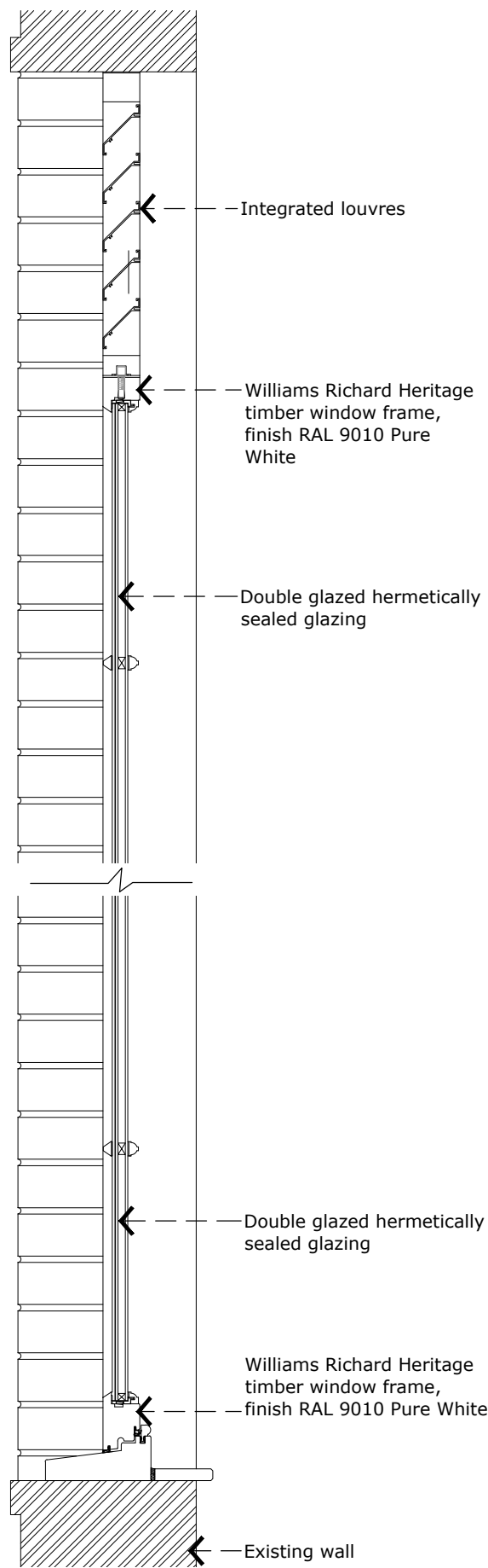
Detail A 1:10
