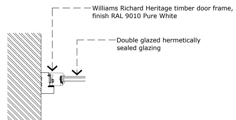
Detail B 1:10
