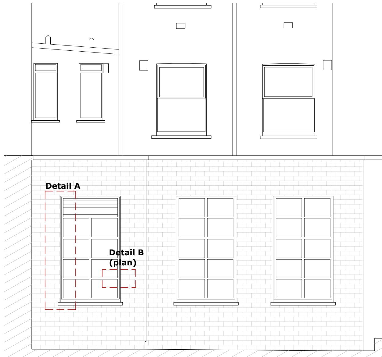
Part Elevation (North East - Rear) 1:50
