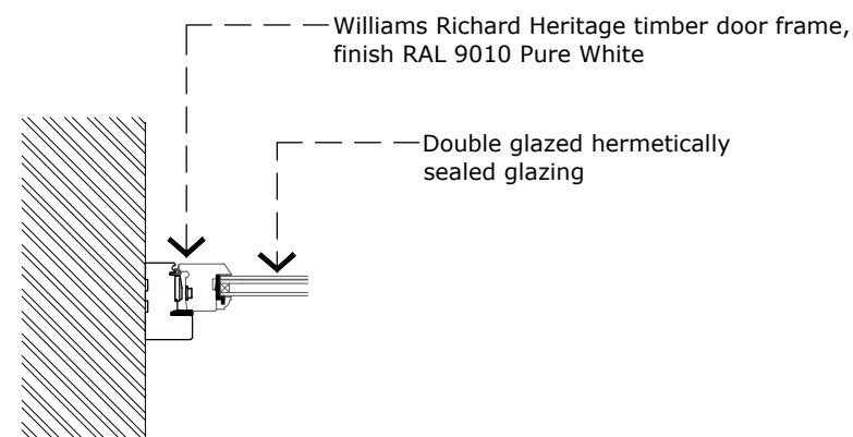
Detail B 1:10
