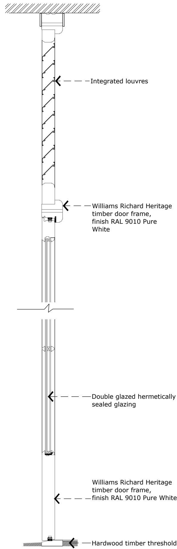
Detail A 1:10
