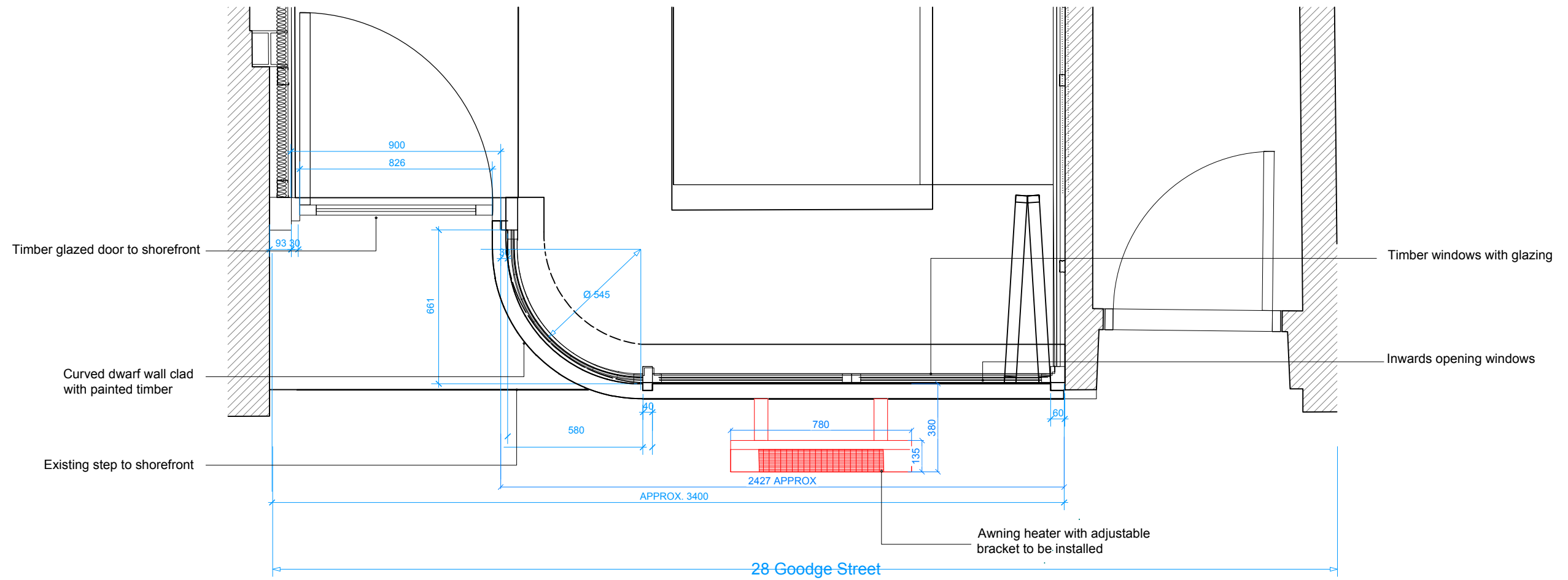
1 Proposed Shop Front Plan 1:20@ A3
