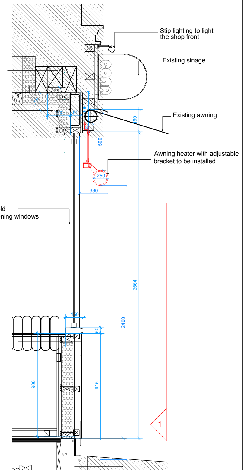
2 Typical Shop Front Section 1:20@ A3
