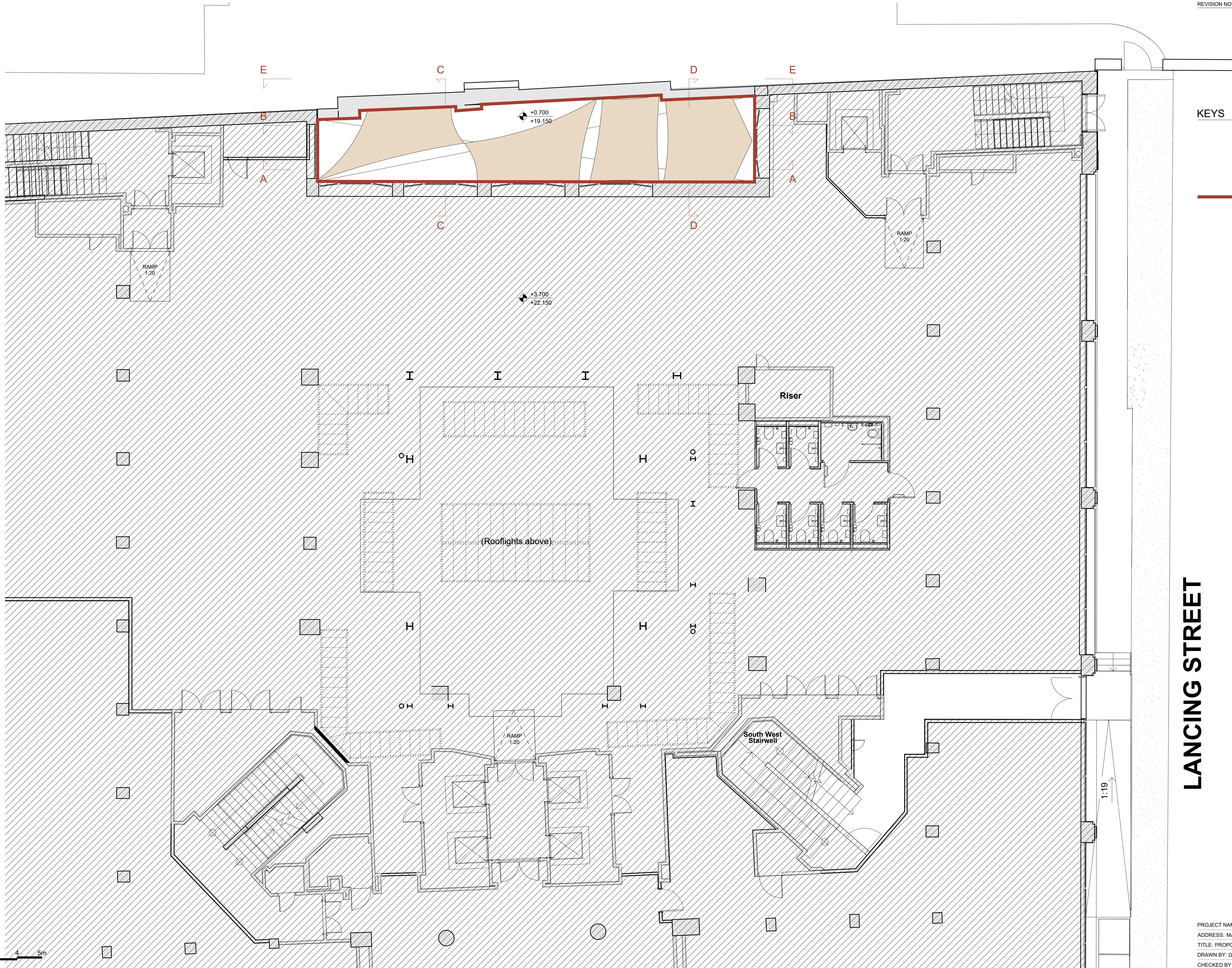
1R EUSTON MAINFRAME - PROPOSED GF GA PLAN SCALE 1:75@ A1 1:150@A3
