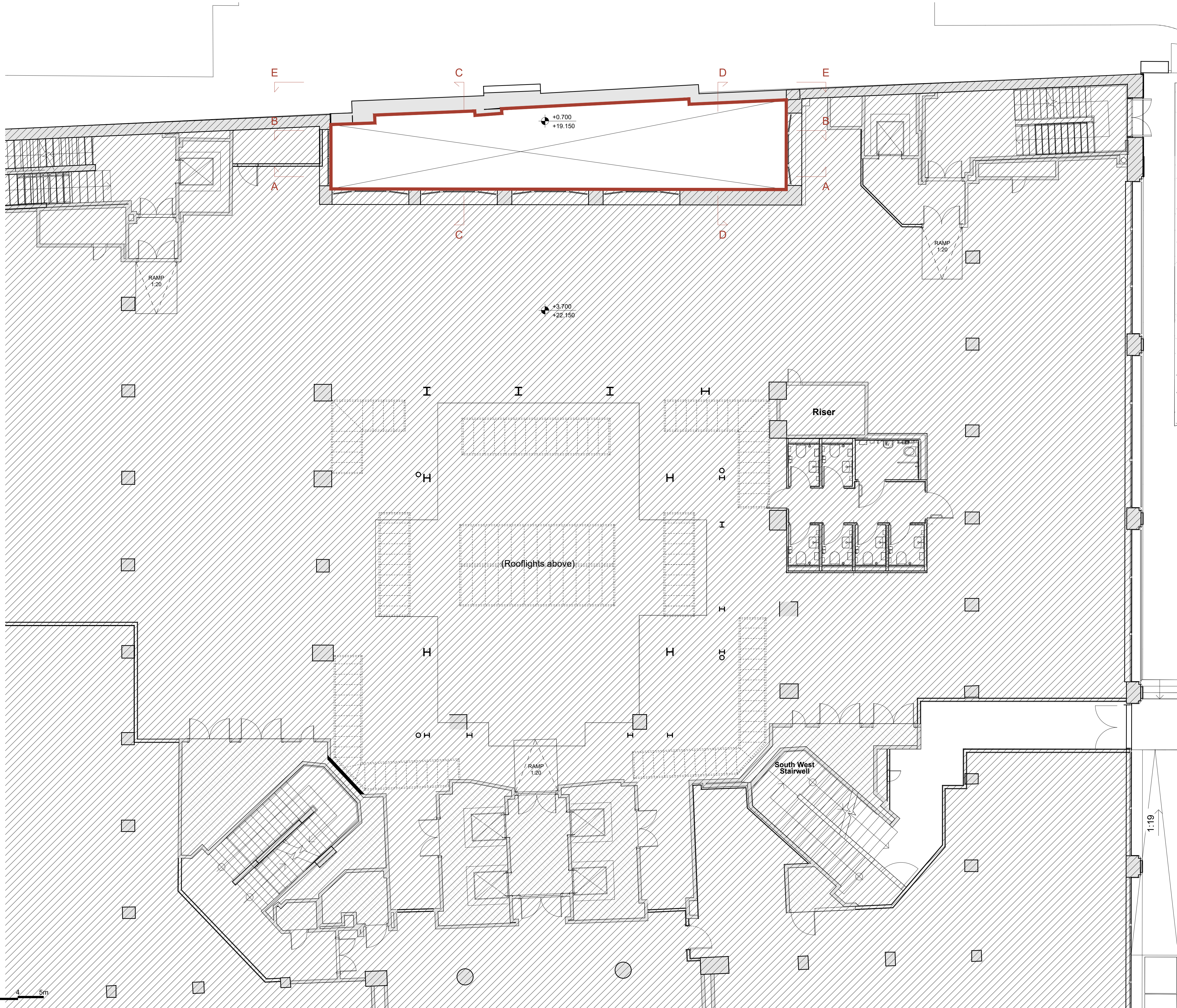
1R EUSTON MAINFRAME - EXISTING GF GA PLAN SCALE 1:75@ A1 1:150@A3
