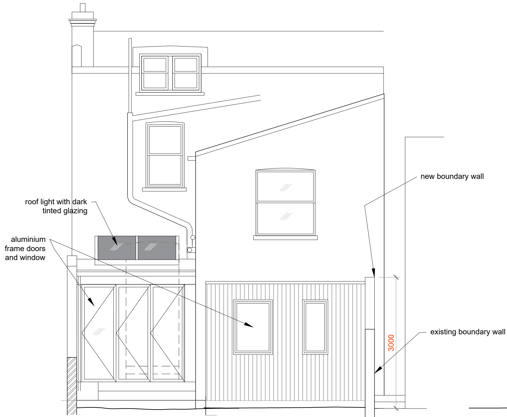
Rear elevation
