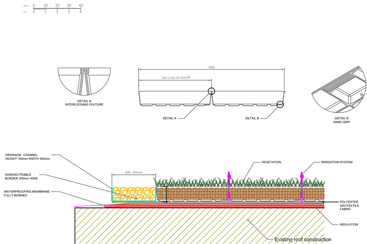
Figure 02 M-TRAY SYSTEM BUILD-UP NTS
