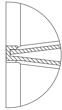
DETAIL A INTERLOCKING FEATURE
