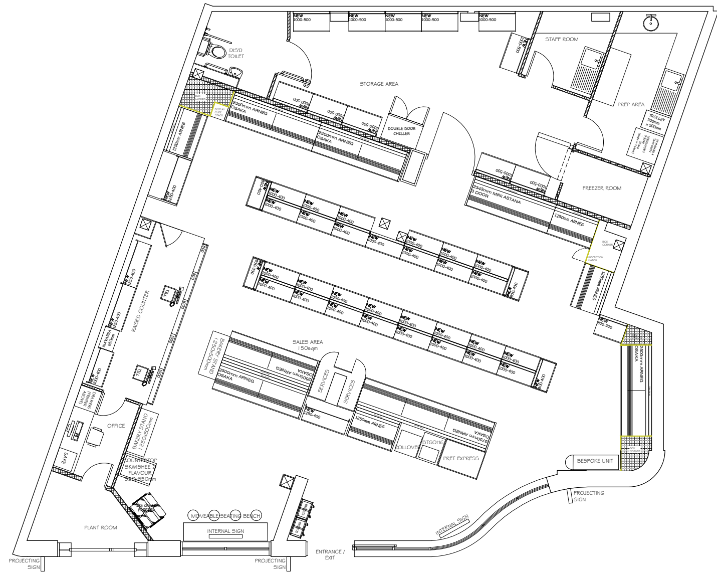
PROPOSED GROUND FLOOR PLAN SCALE 1:50@A1
