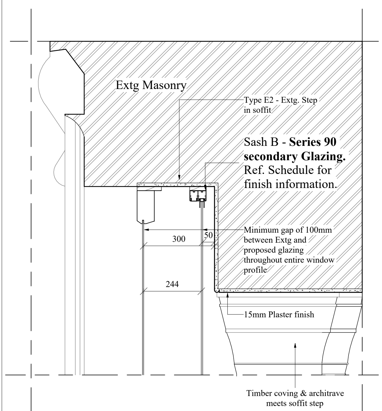
TYPE E2: PROPOSED SECTION (details elsewhere repeated as E1)
