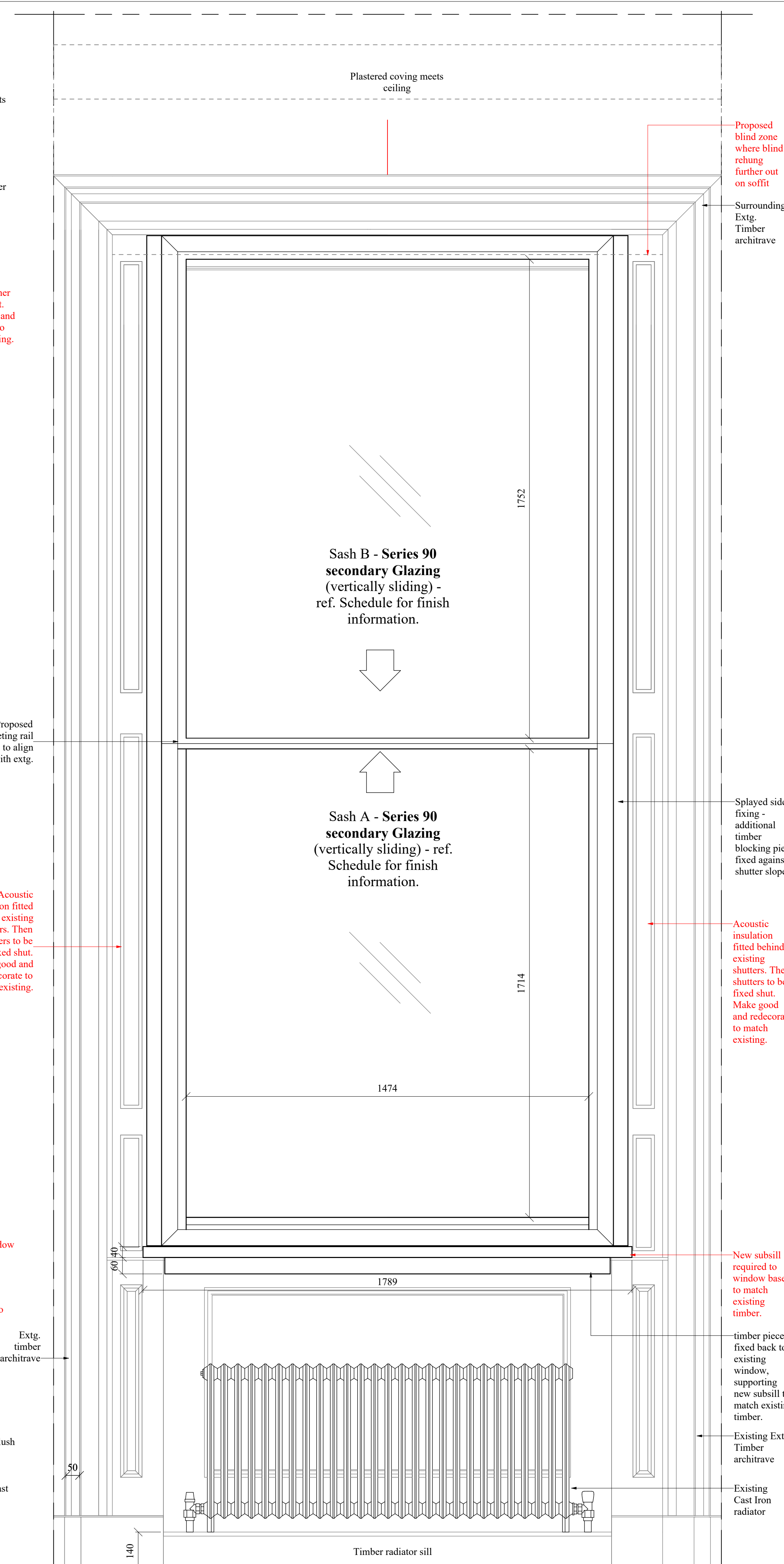
TYPE E1: PROPOSED ELEVATION
