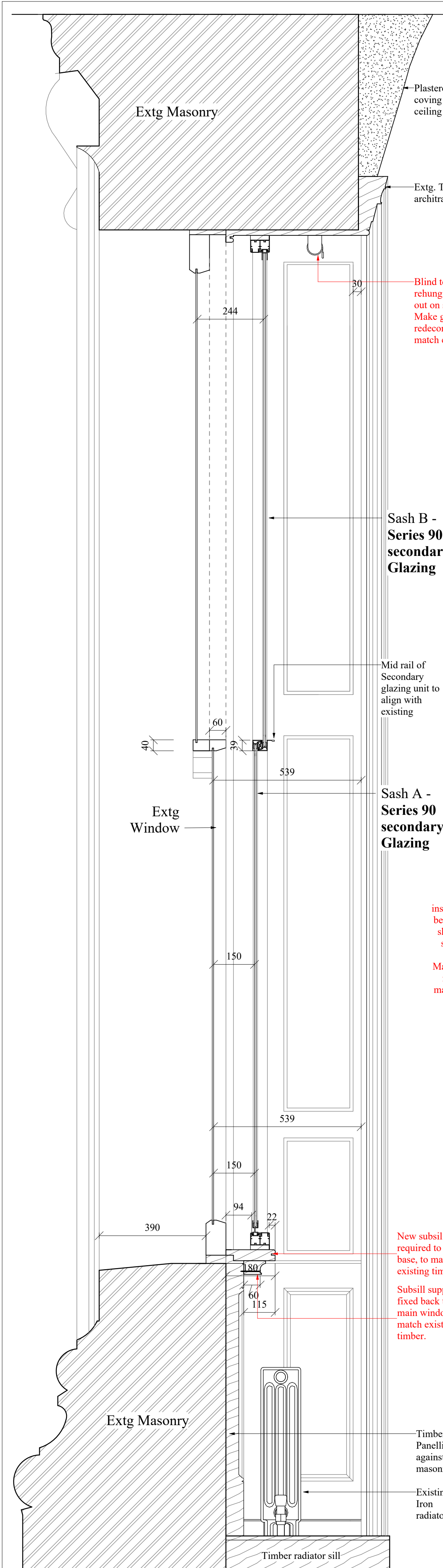
TYPE E1: PROPOSED SECTION
