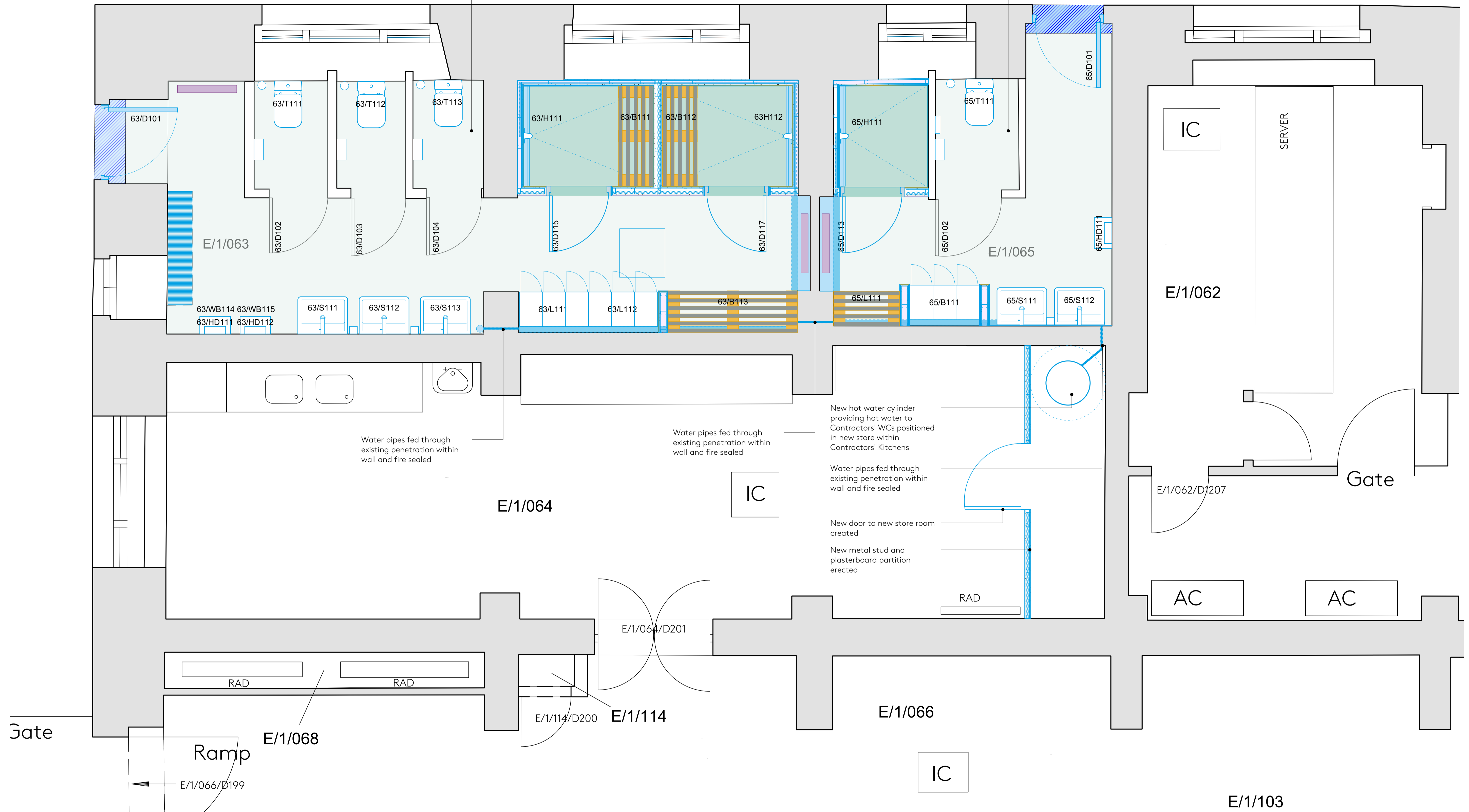
1 Contractor Toilet Facilities 1F Plan - Proposed Scale: 1:25
