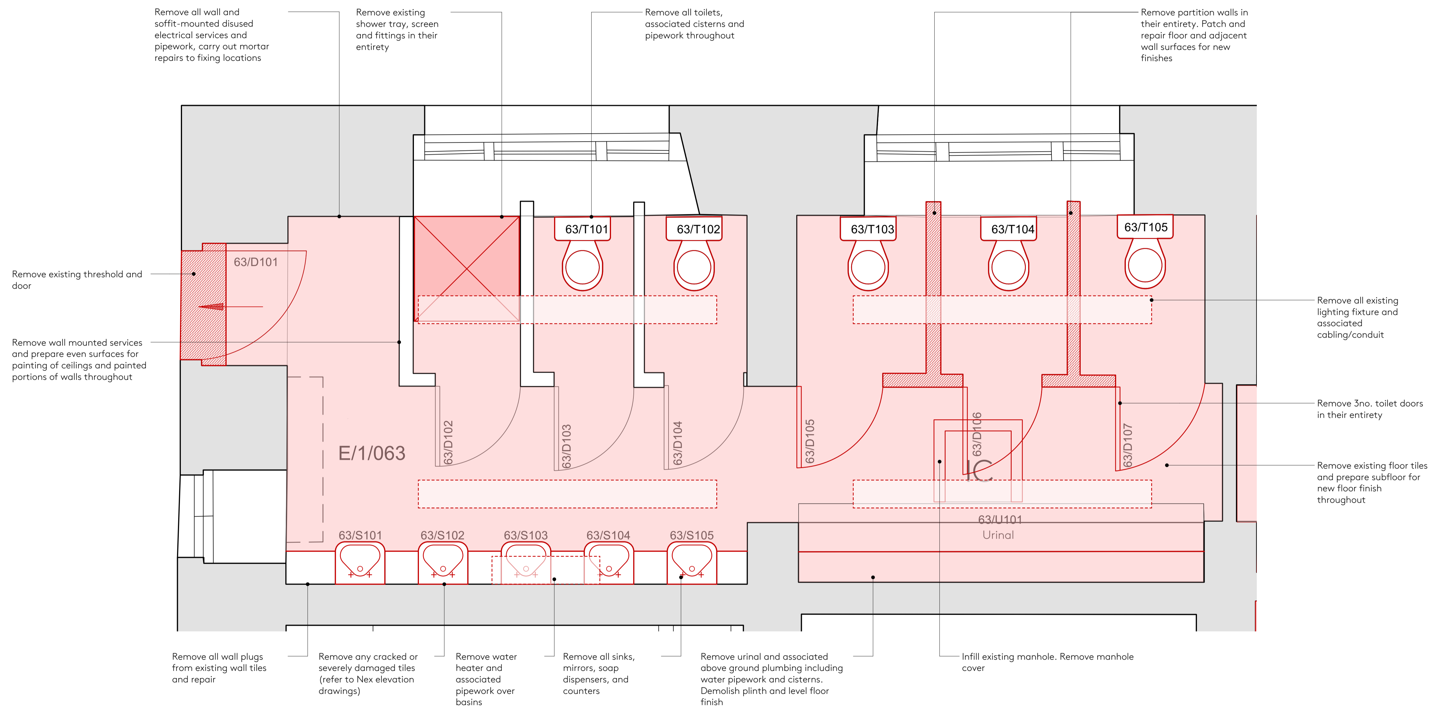
1 Male WC Plan - Existing & Demolition Scale: 1:20
