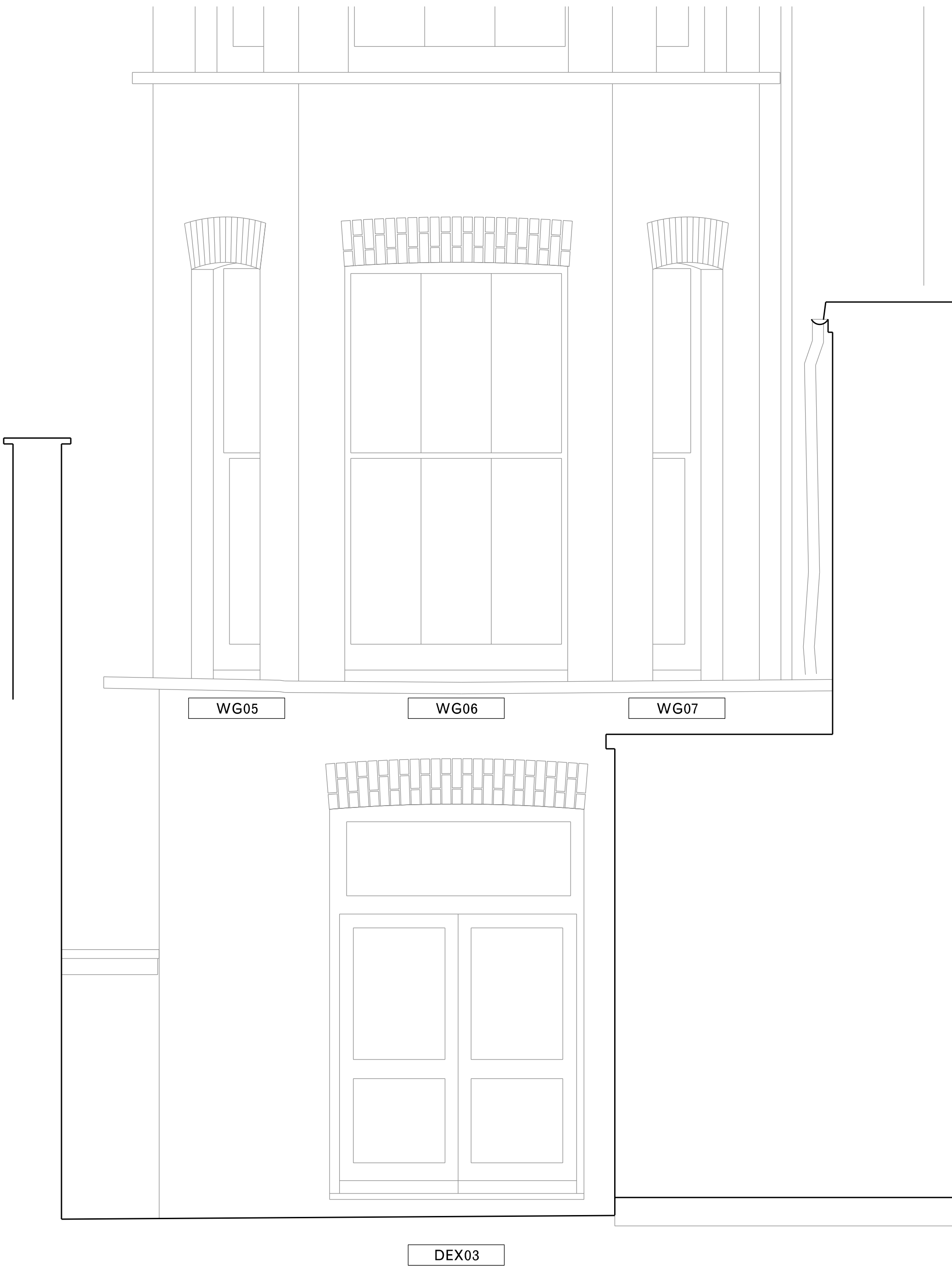
01 Rear facade elevation Scale 1:25
