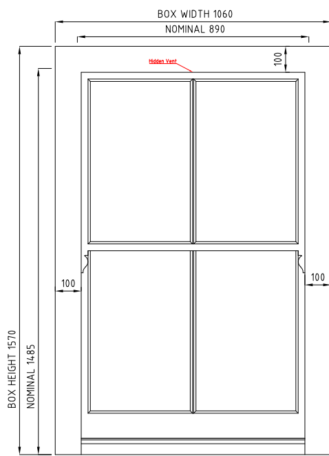
BOX SASH WINDOW VIEWED FROM OUTSIDE SCALE 1:20 WB.14
