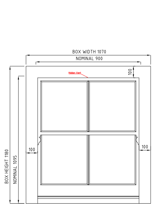
BOX SASH WINDOW VIEWED FROM OUTSIDE SCALE 1:20 WG.11/WG.12
