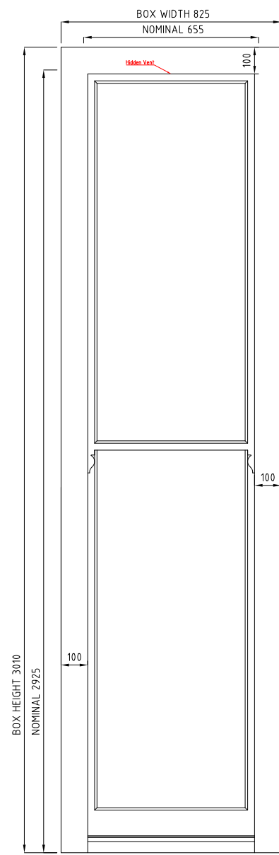
BOX SASH WINDOW VIEWED FROM OUTSIDE SCALE 1:20 WG.05
