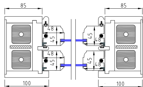
HORIZONTAL SECTION SCALE 1:5
