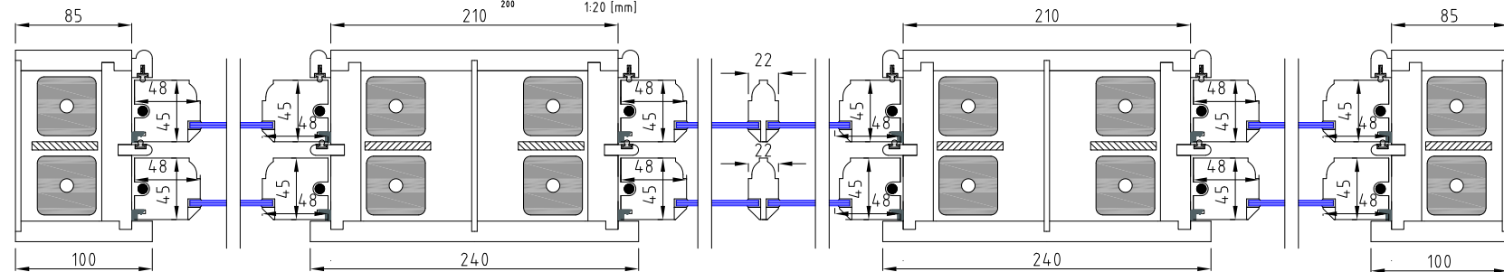
HORIZONTAL SECTION SCALE 1:5
