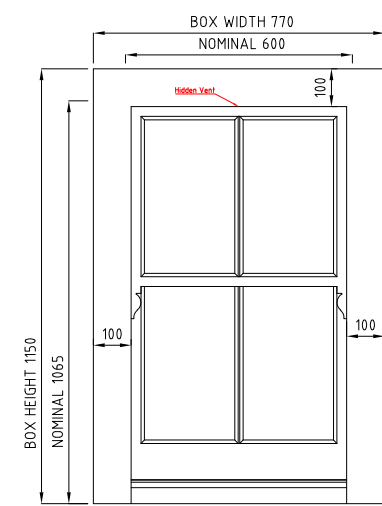
BOX SASH WINDOW VIEWED FROM OUTSIDE SCALE 1:20 WB.12
