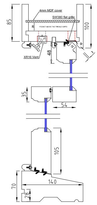
VERTICAL SECTION SCALE 1:5
