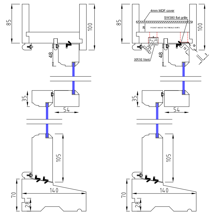
VERTICAL SECTION SCALE 1:5
