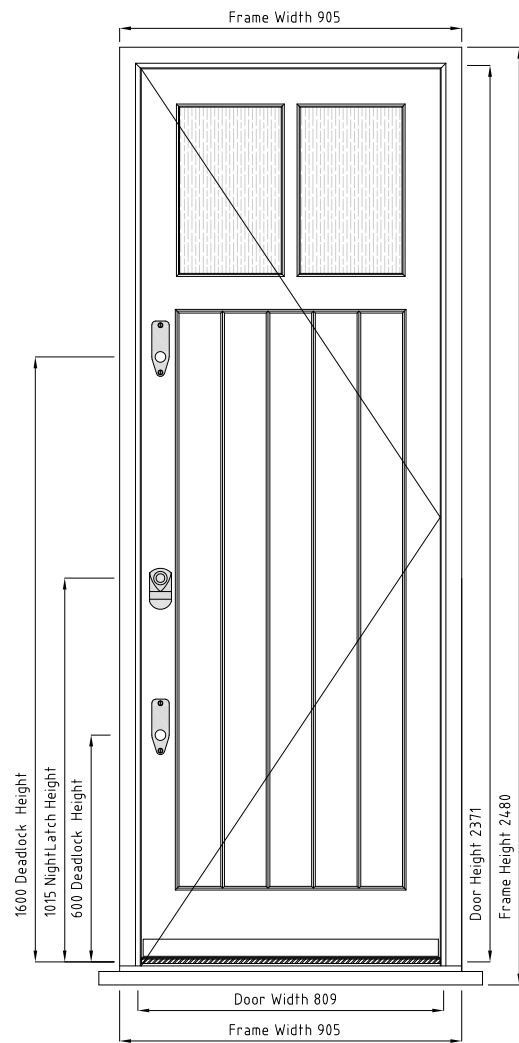
DEX.06 Doors viewed from outside Doors open inwards Scale 1:20
