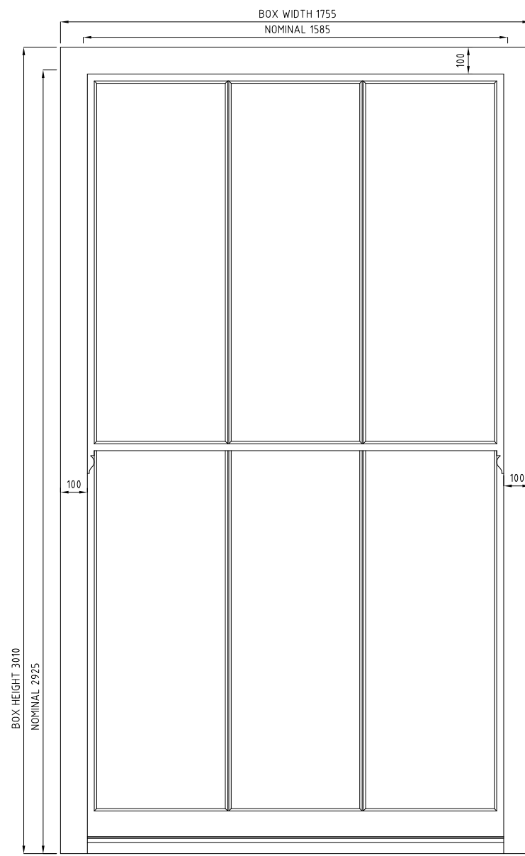
BOX SASH WINDOW VIEWED FROM OUTSIDE SCALE 1:20 WG.06
