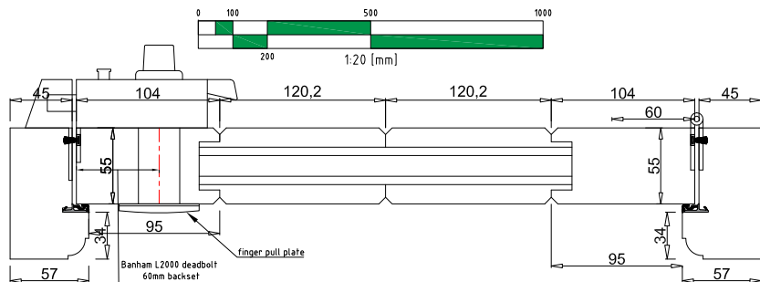
DEX.06 Doors viewed from outside Doors open inwards Scale 1:20
