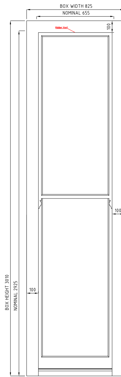
BOX SASH WINDOW VIEWED FROM OUTSIDE SCALE 1:20 WG.07
