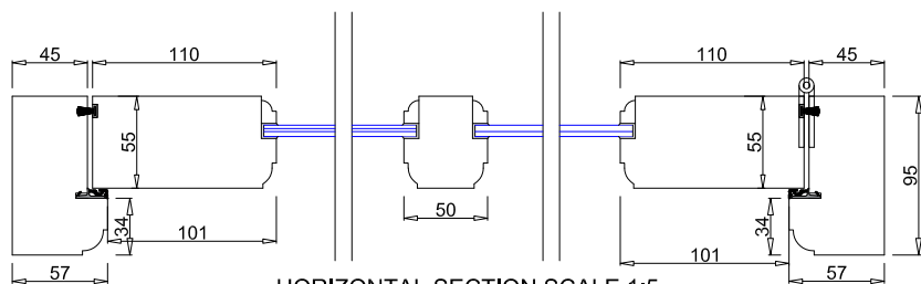
HORIZONTAL SECTION SCALE 1:5
