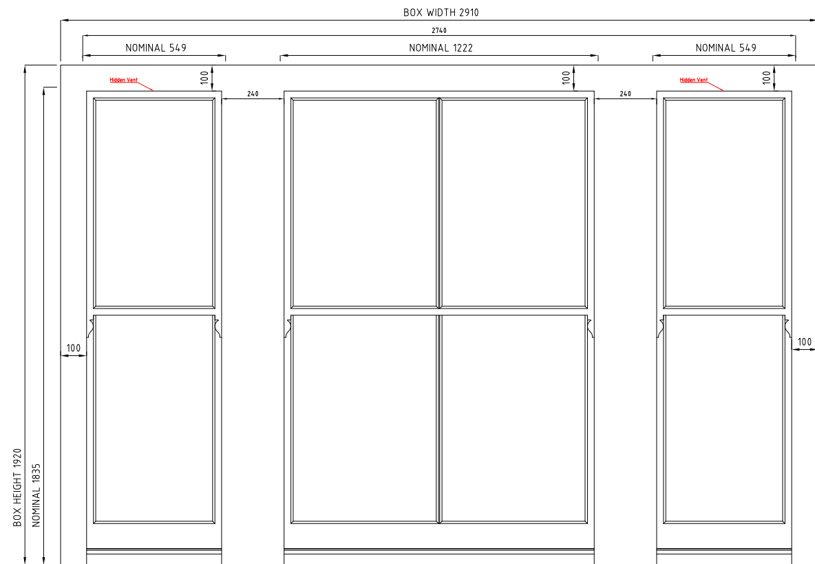
BOX SASH WINDOW VIEWED FROM OUTSIDE SCALE 1:20 WB.03 / WB.02 / WB.01
