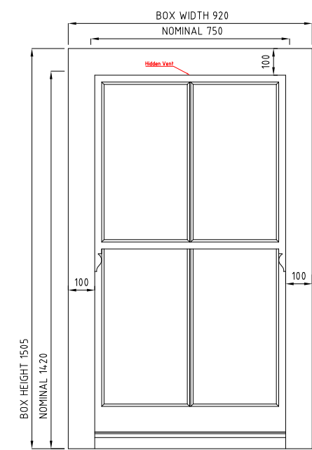
BOX SASH WINDOW VIEWED FROM OUTSIDE SCALE 1:20 WG.13/WG.14/WG.15/WG.16
