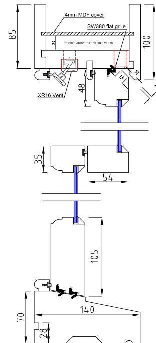
VERTICAL SECTION SCALE 1:5
