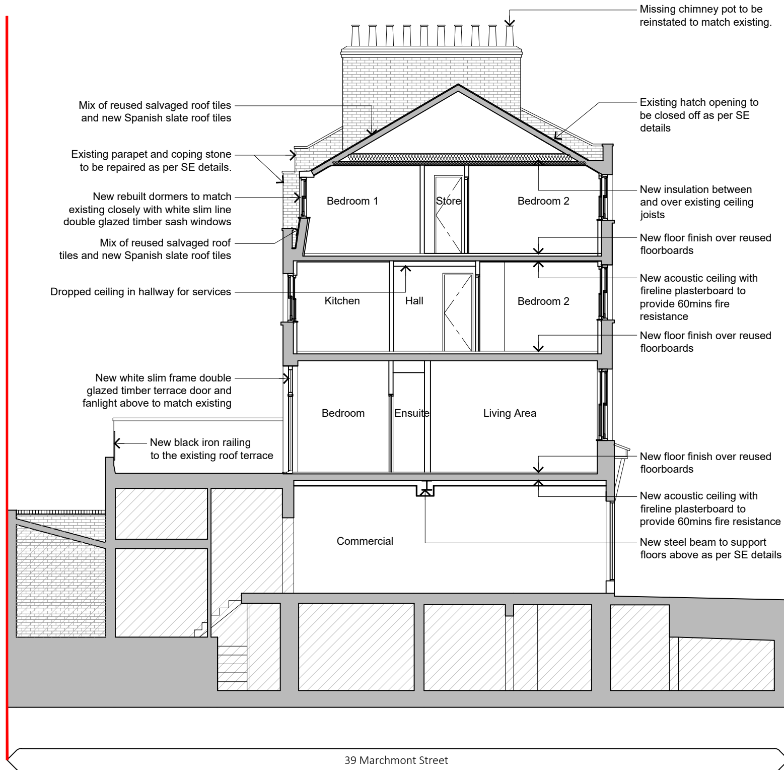
1 Proposed Section A-A 1:100 @ A3 (1:50@A1)
