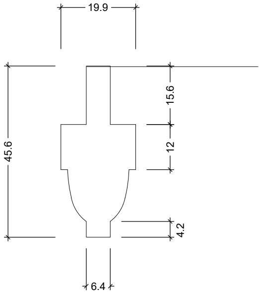
02 Glazing bar profile detail - Window Type F3.1, F3.2, R3.1 and R3.2 1:1@A3
