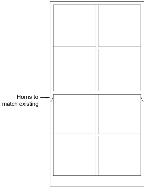
03 Window Elevation 1:20@A3
