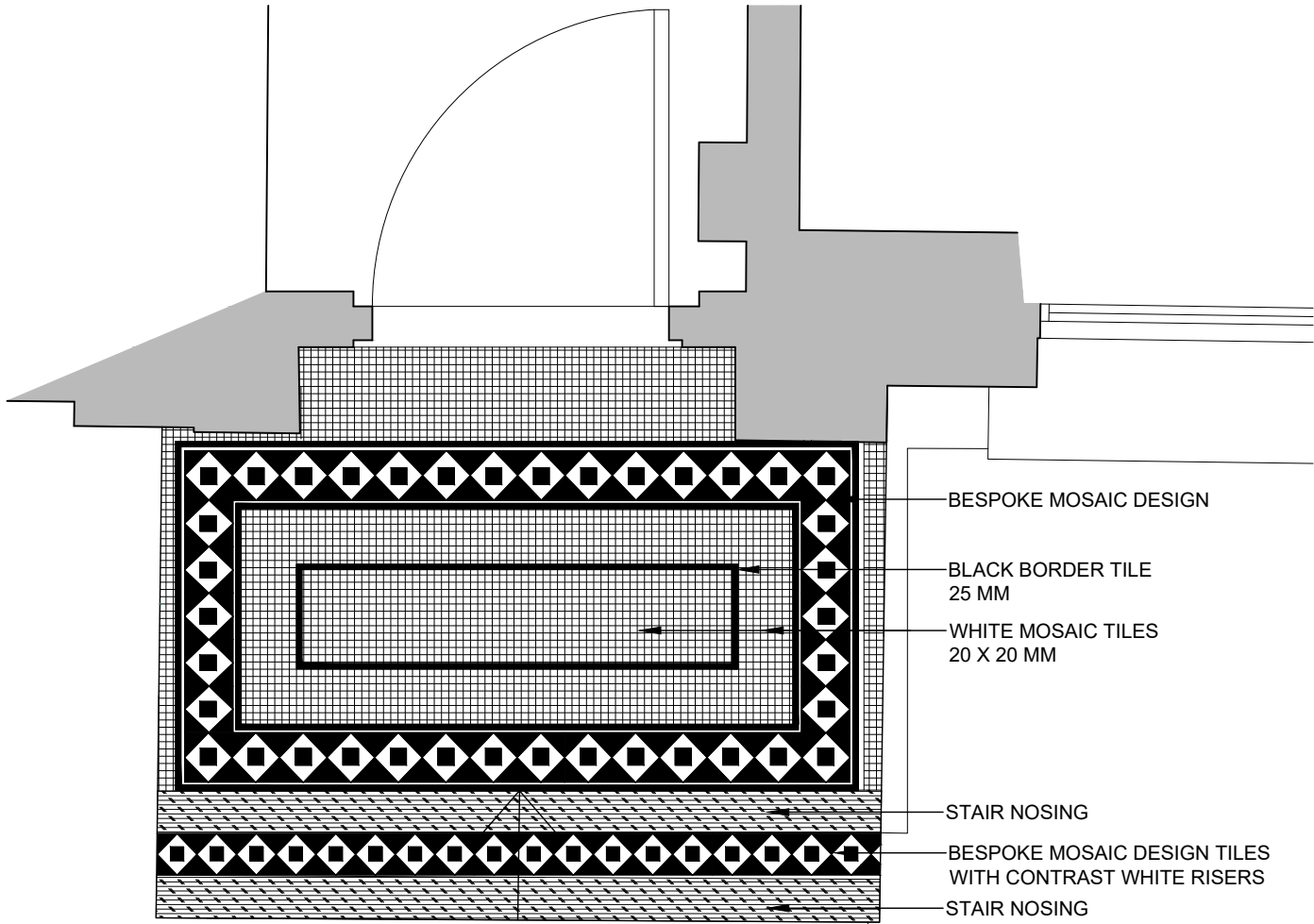
BESPOKE TILES SETTING OUT 1@25
