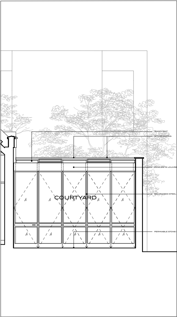
SECTION CC
