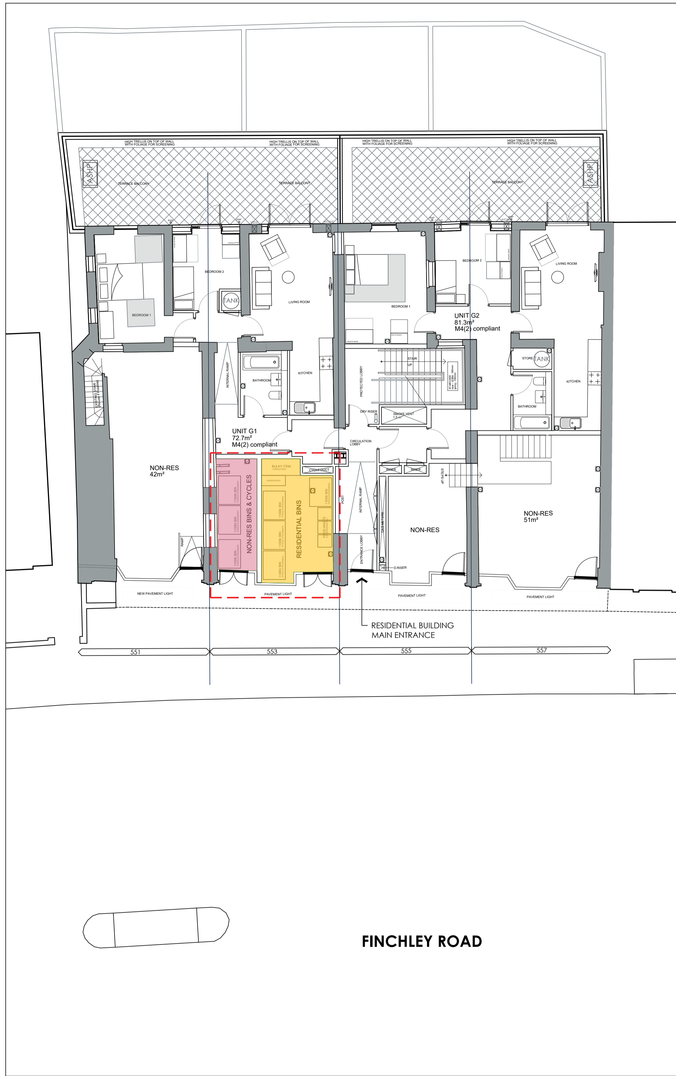
1 GROUND FLOOR - BIN/CYCLE STORAGE LOCATION Scale: 1:200
