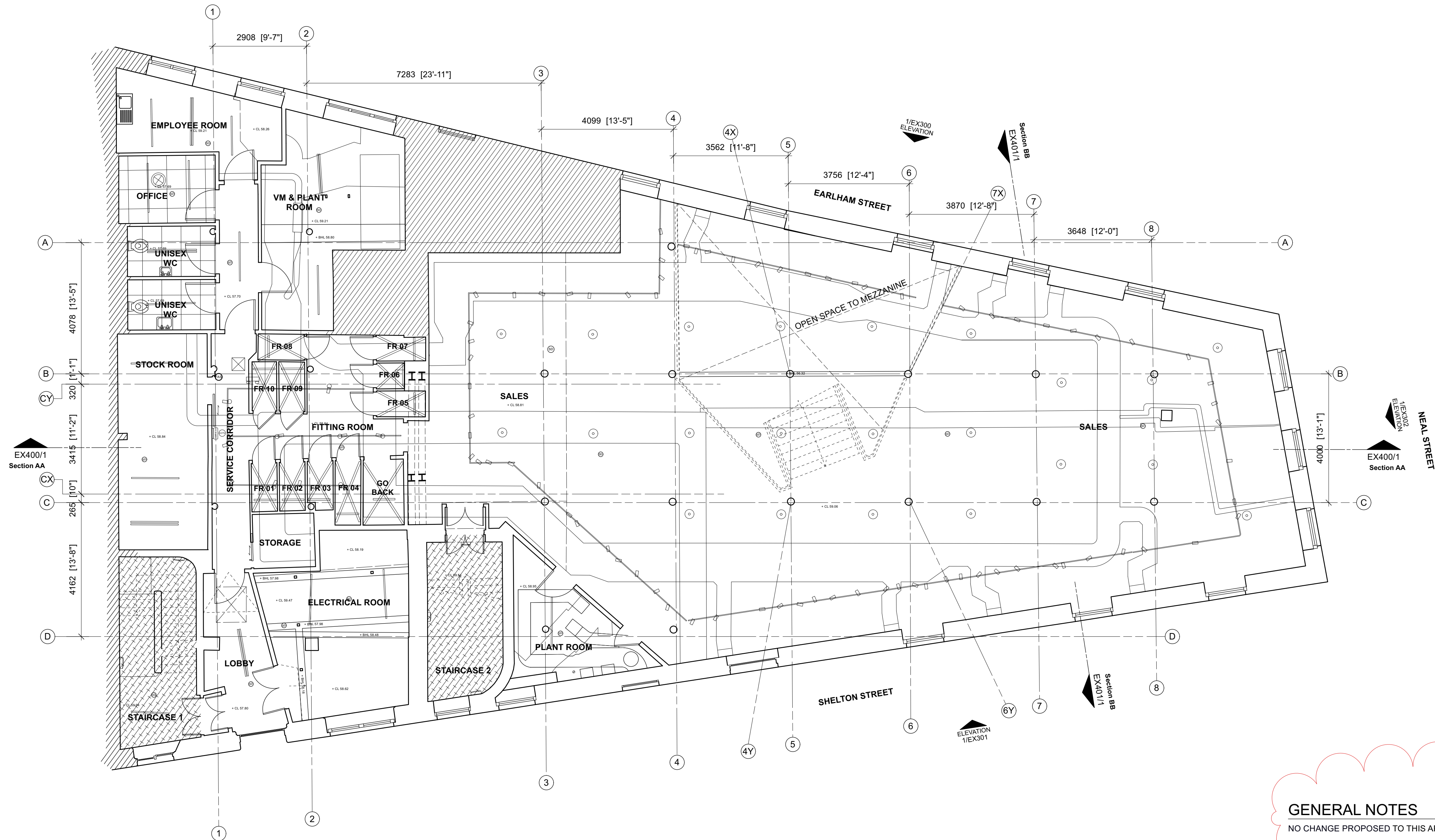
1 FIRST FLOOR RCP
