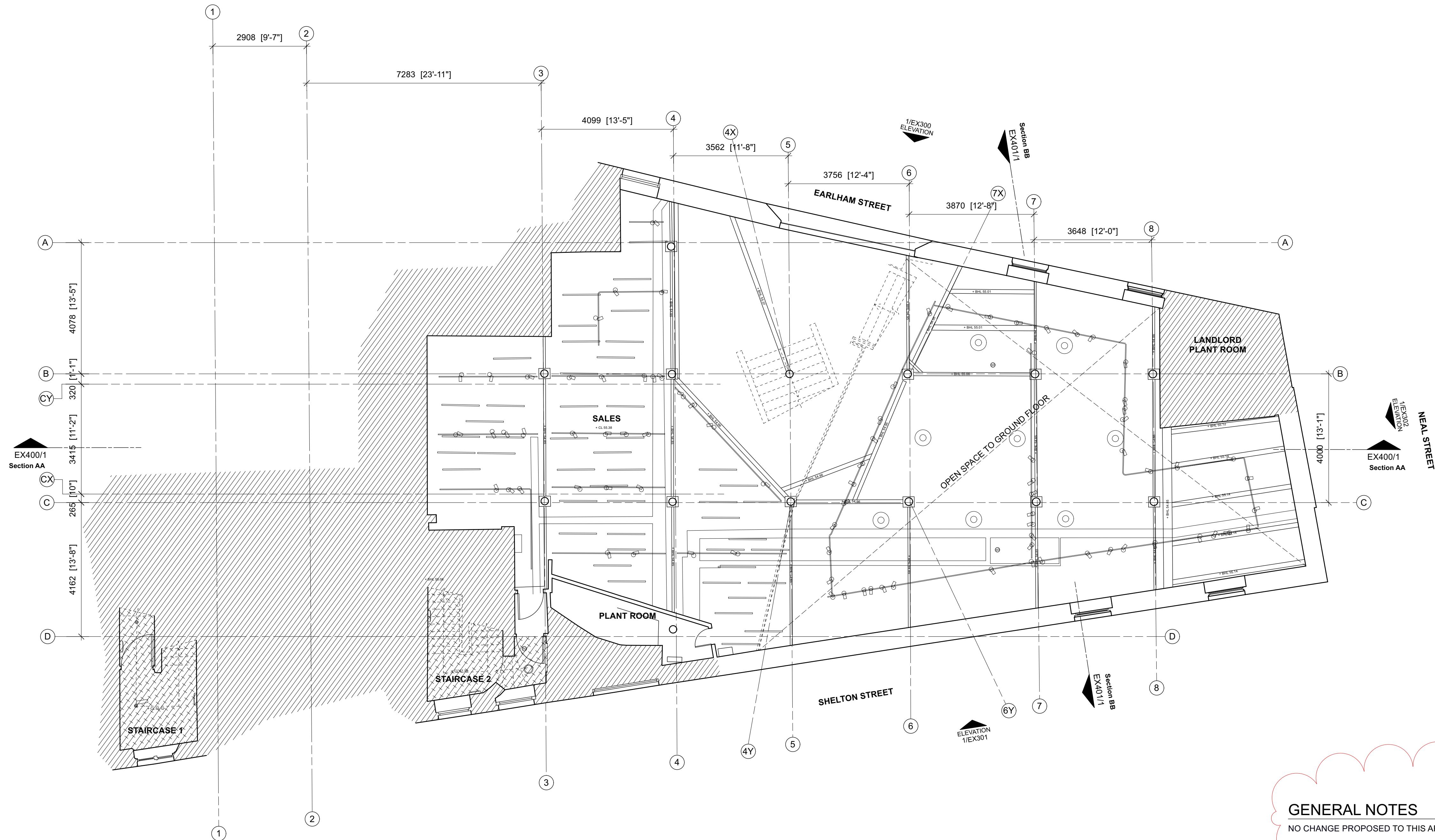
1 MEZZANINE FLOOR RCP EX201 SCALE 1:75 @ A1
