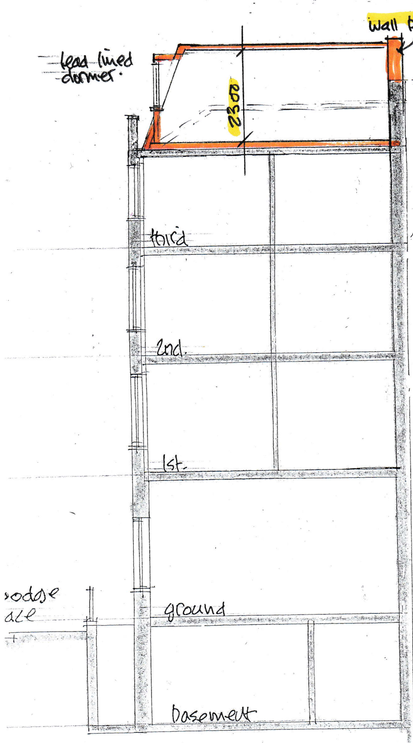
SECTION BB.
