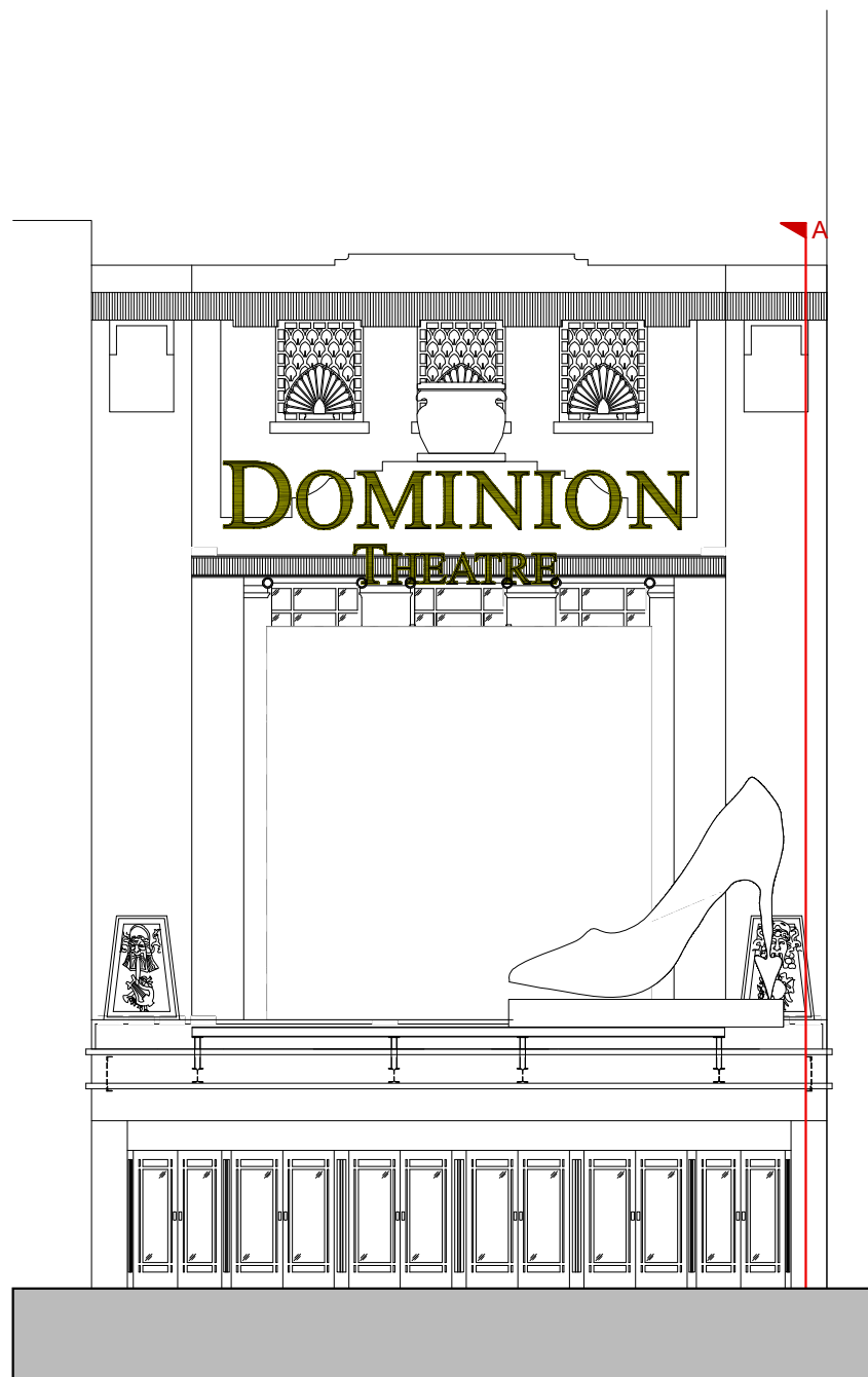
Existing Front Elevation (Scale 1:100 @ A3)
