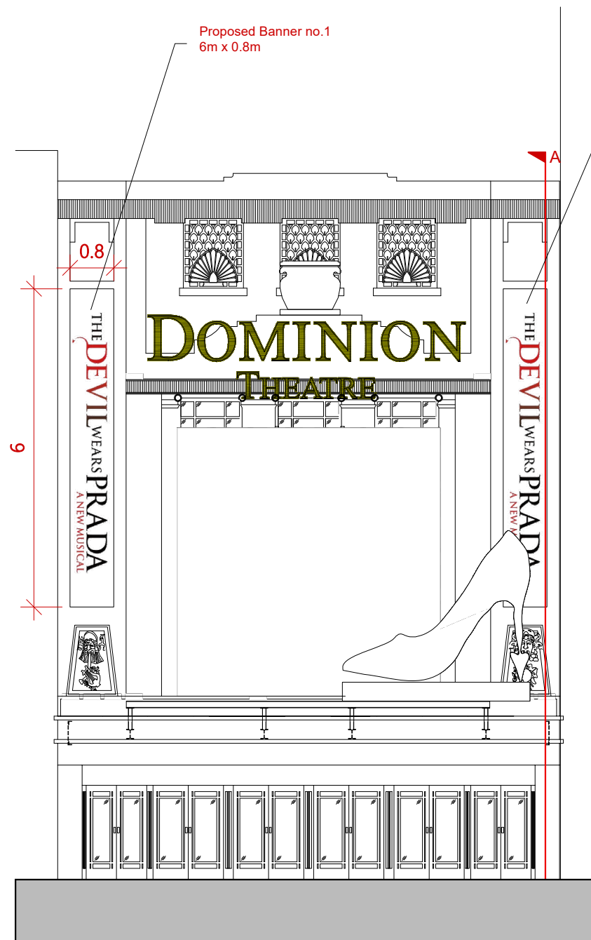
Proposed Front Elevation (Scale 1:100 @ A3)
