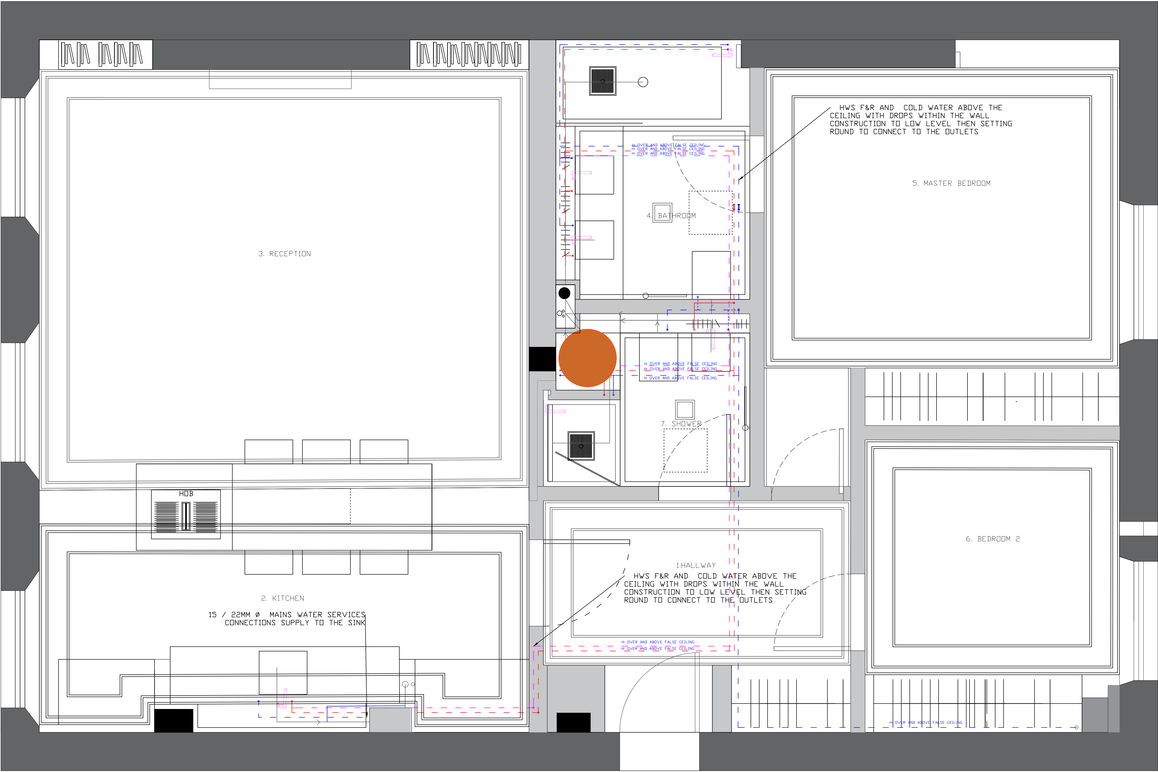
PLAN DETAILING THE DOMESTIC SERVICES LAYOUT
