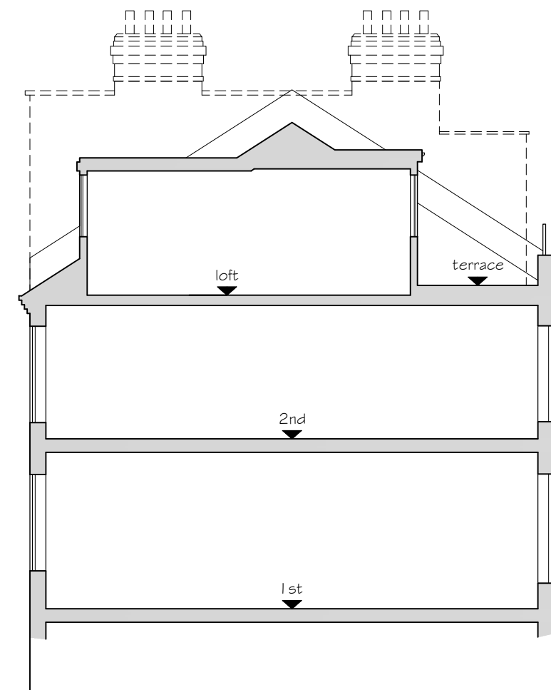
Part Section [existing] 1:100
