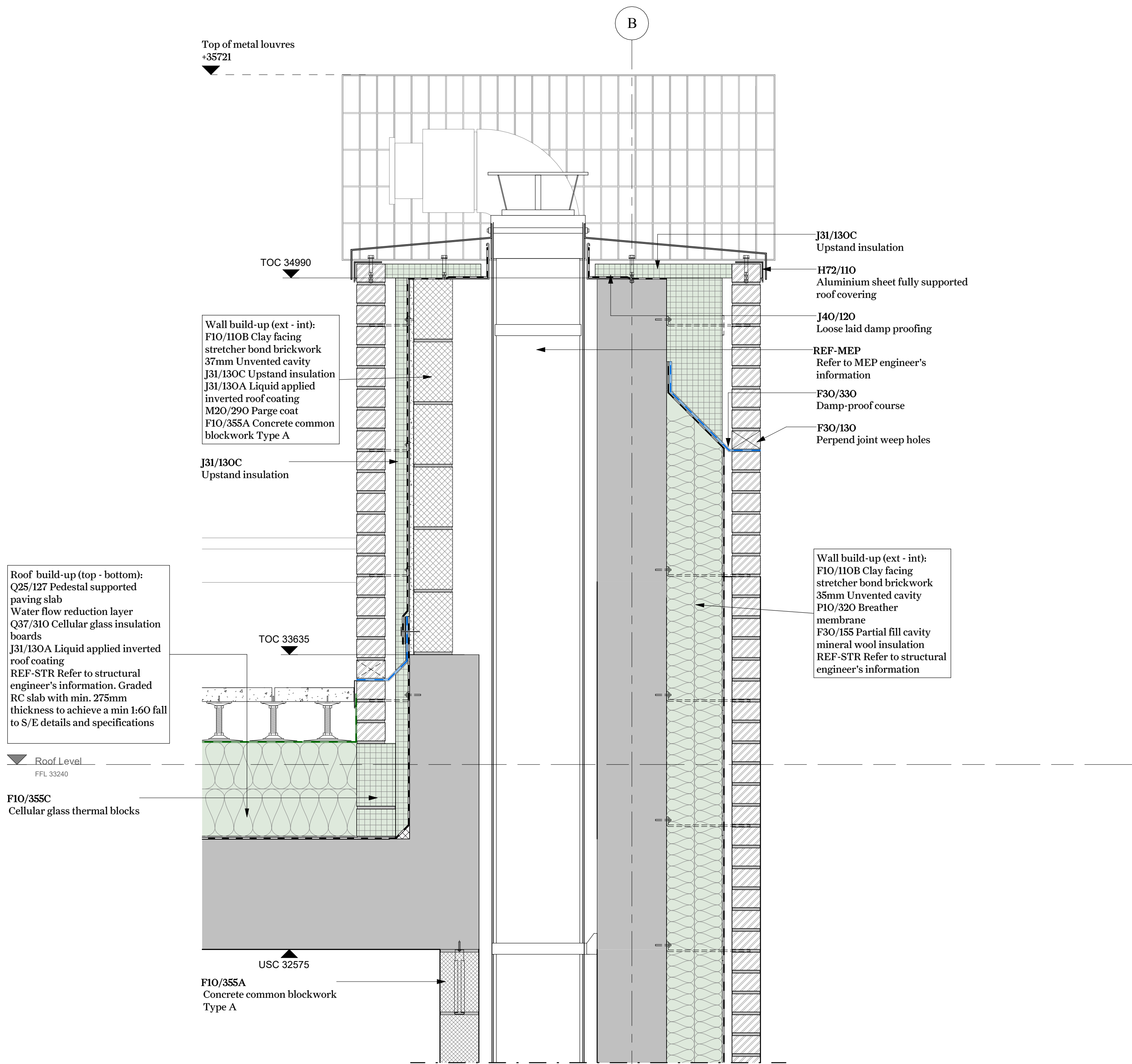
1 North Parapet Wall and Chimney Detail 1 : 10
