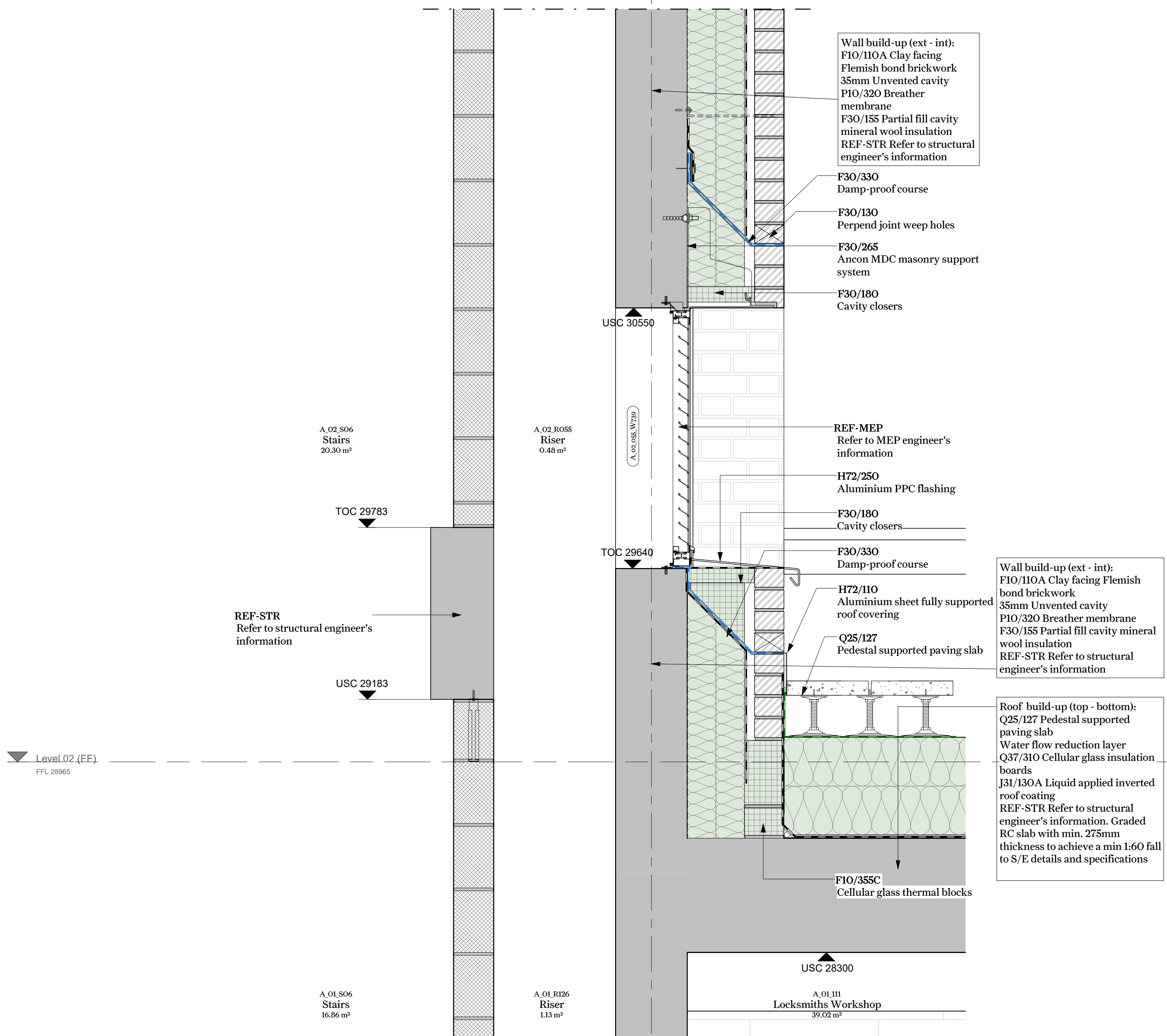
2 North Riser Vent Detail 1 : 10
