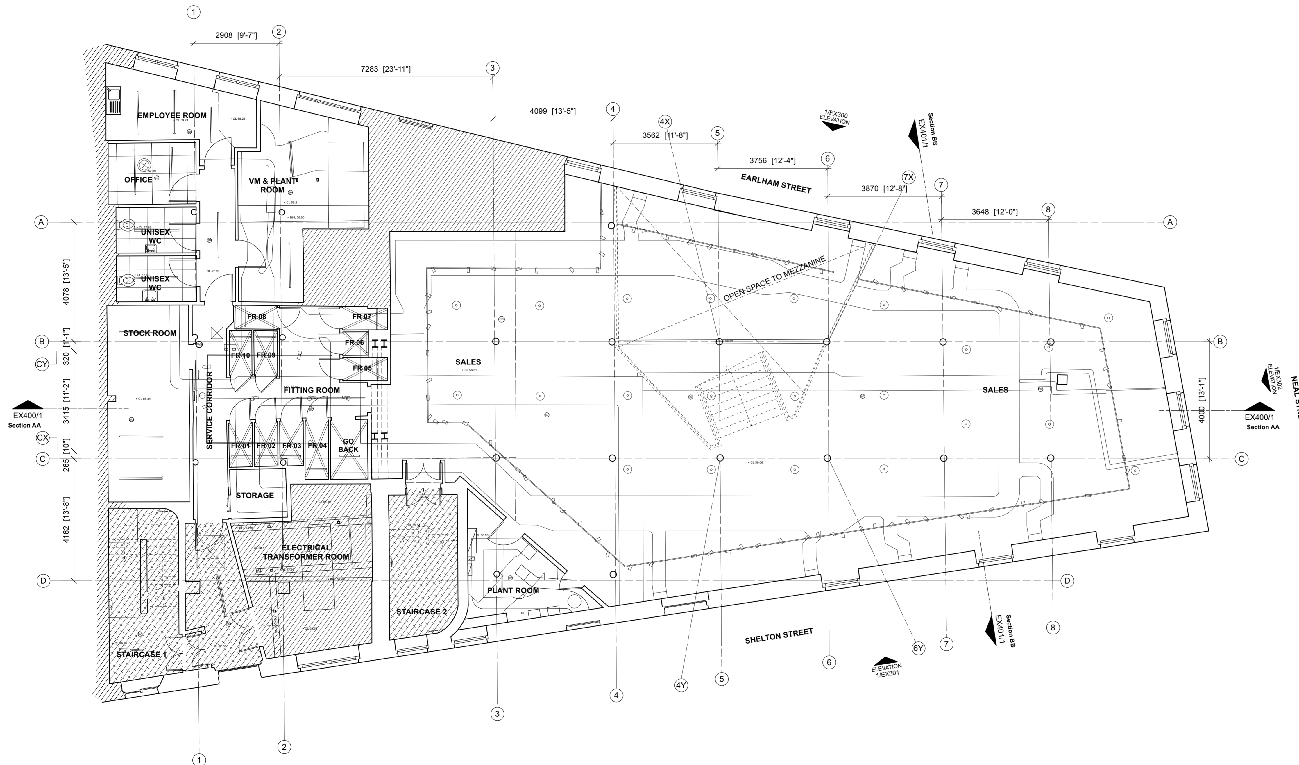
1 FIRST FLOOR RCP EX202 SCALE 1:75 @ A1
