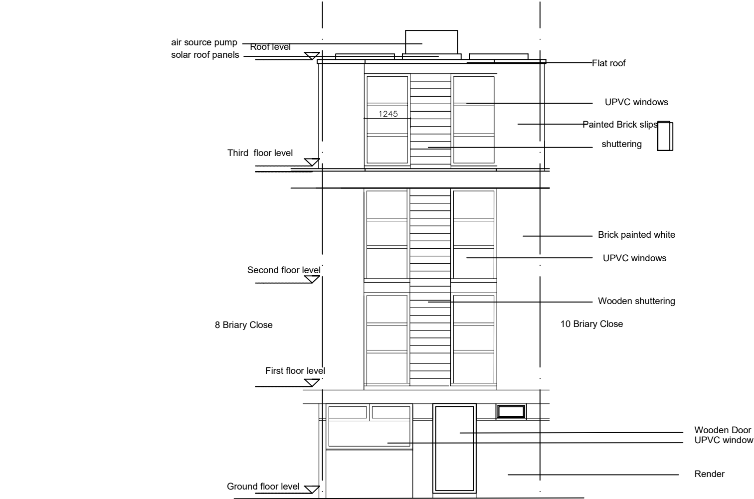
Front Elevation
