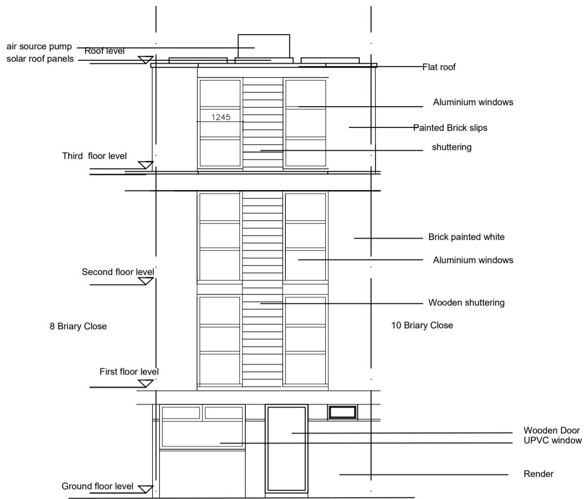
Front Elevation
