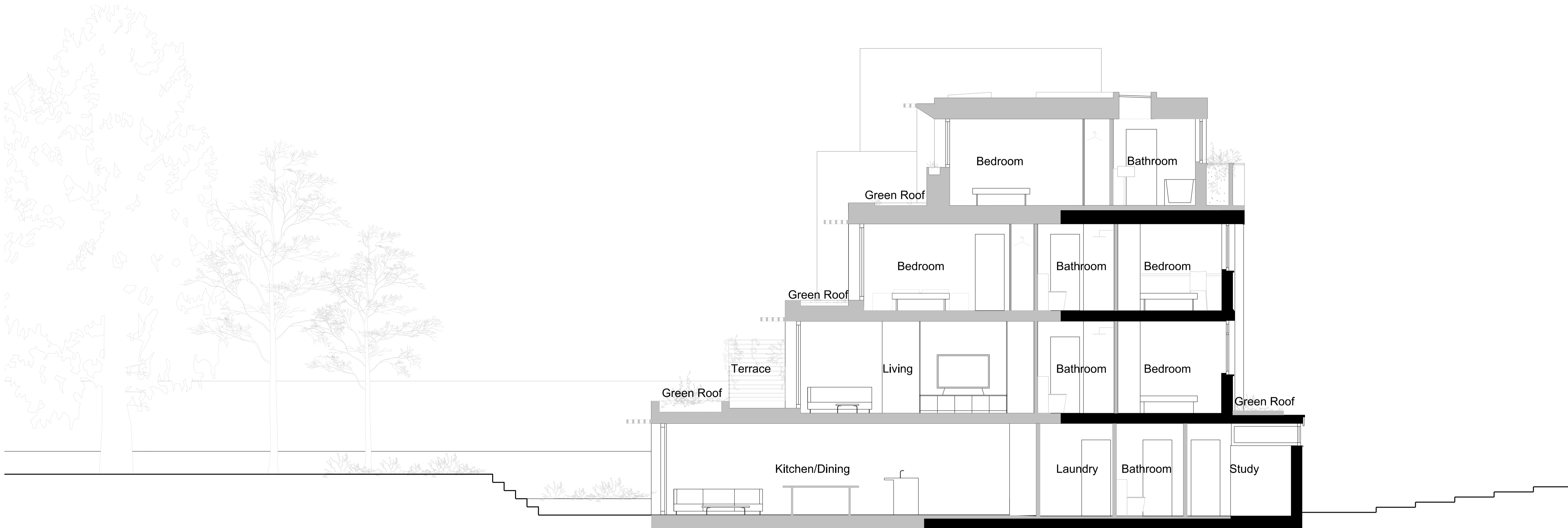
01 Proposed Section Scale 1:50 @ A1
