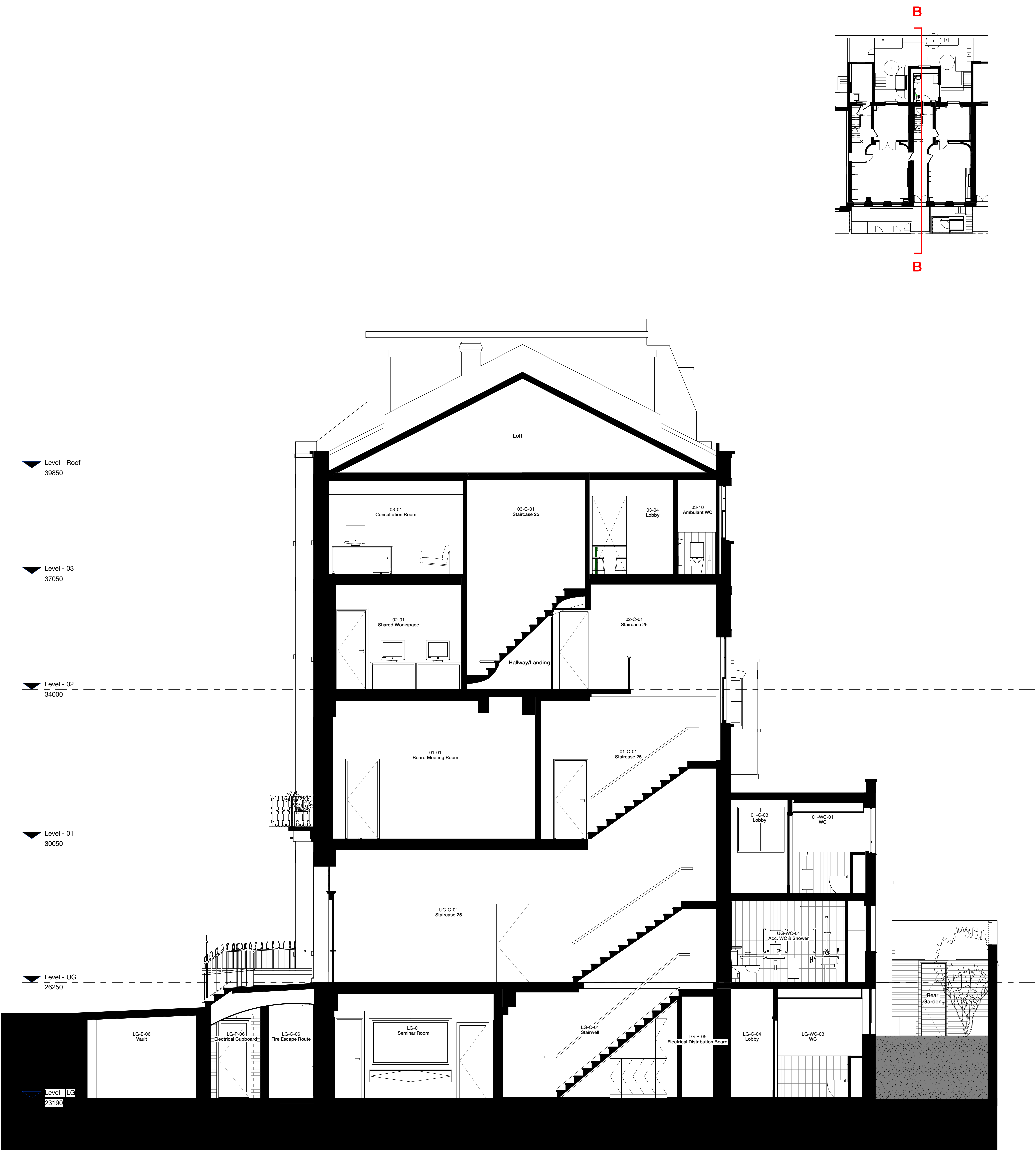
Proposed Section BB (Through 25 Woburn Square)
