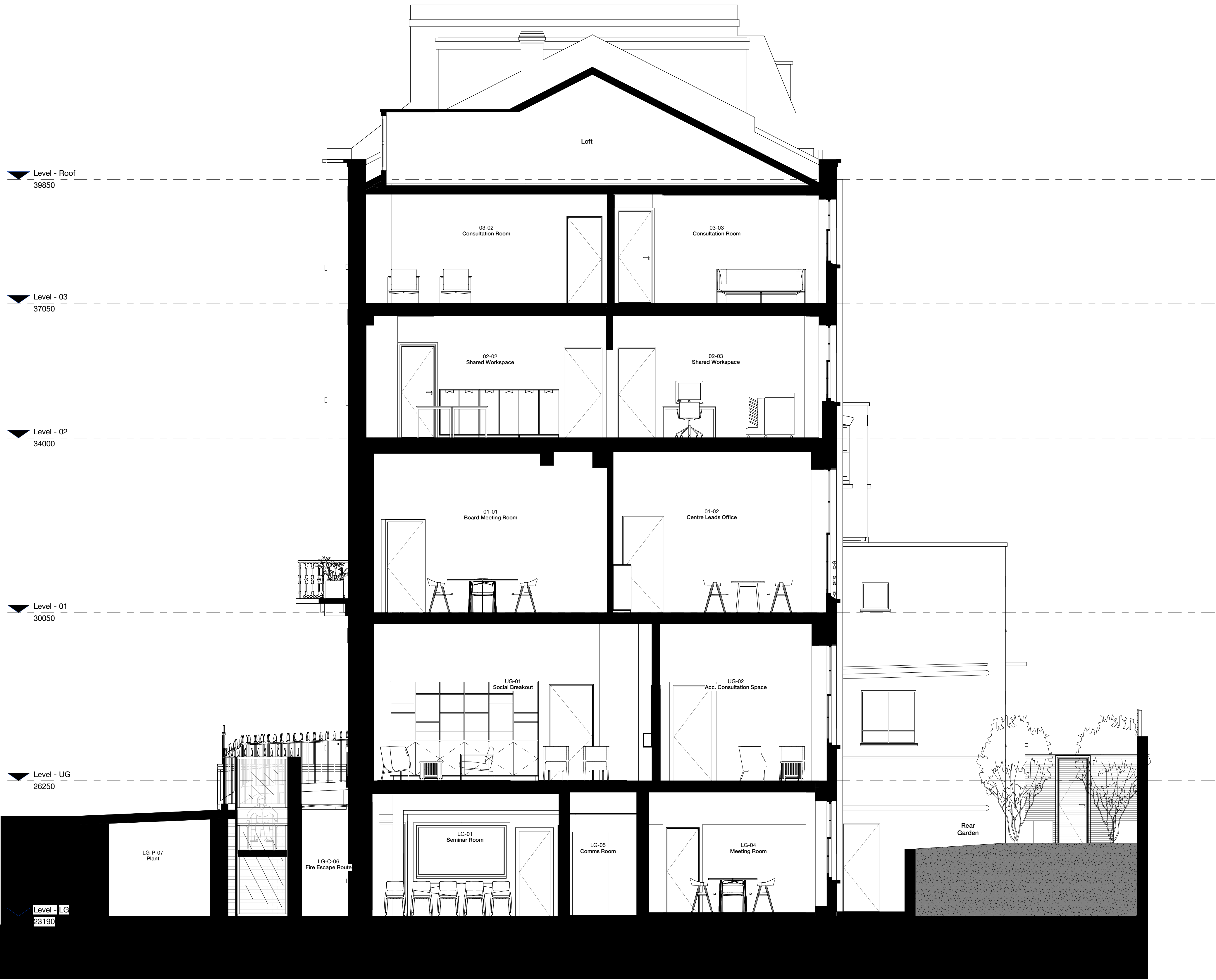
Proposed Section AA (Through 25 Woburn Square)
