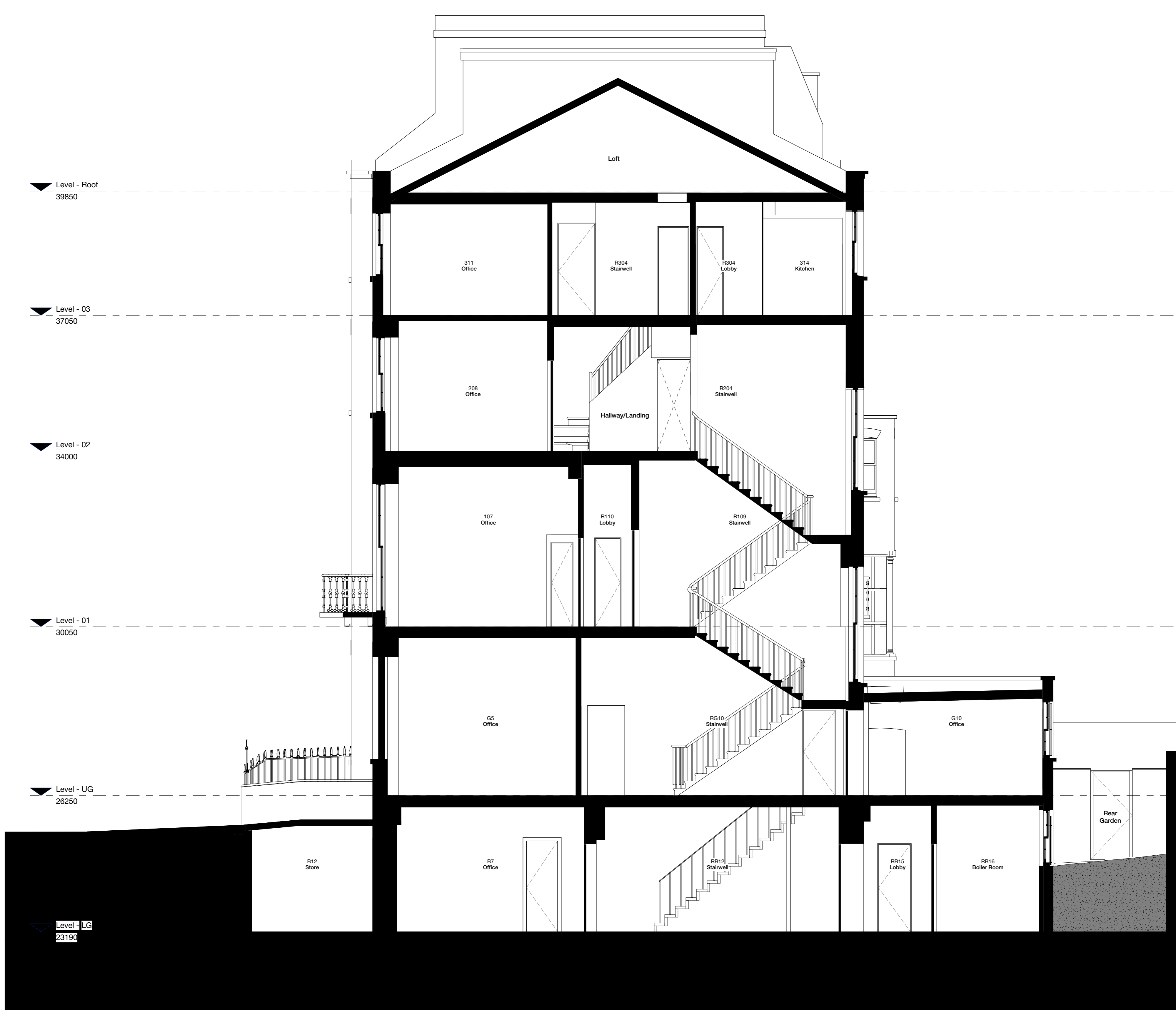
Existing Section DD (26 Woburn Square) 1:50
